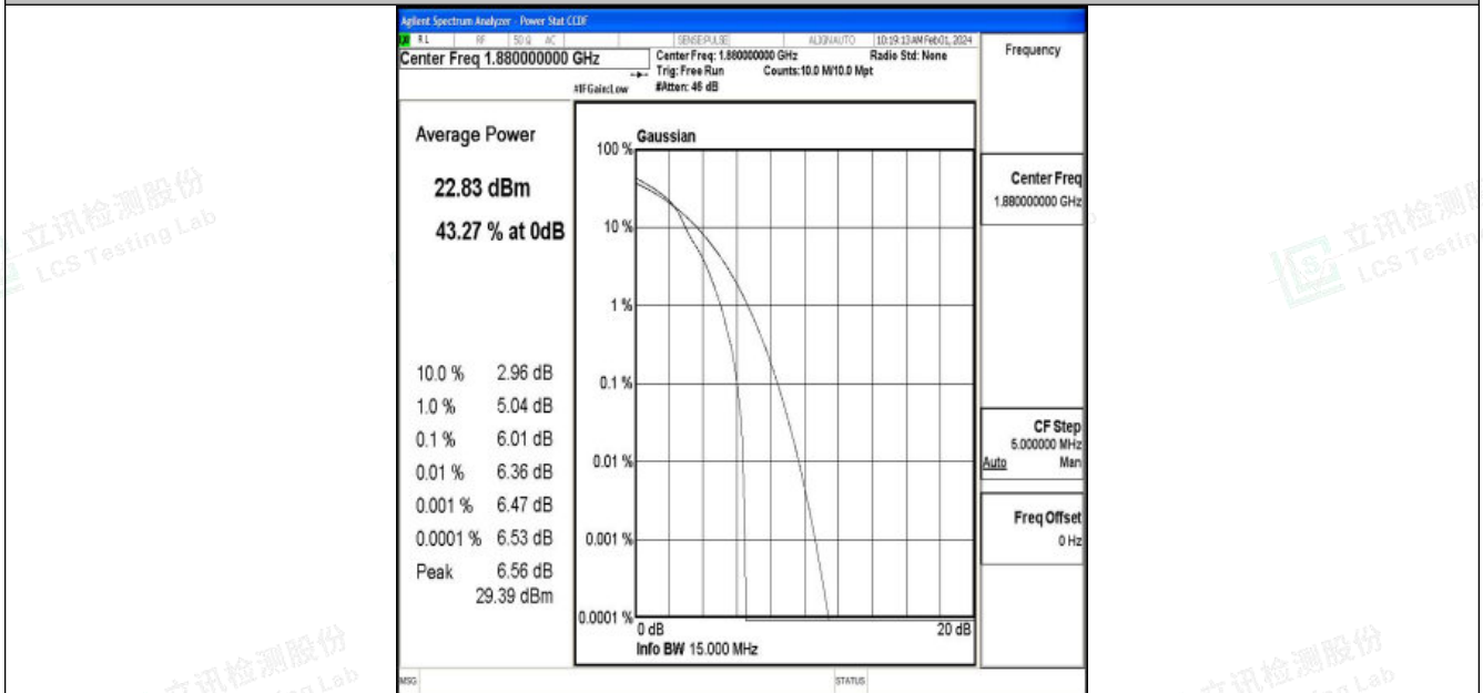
Band2-15MHz-16QAM-18900-1RB#0-PASS
