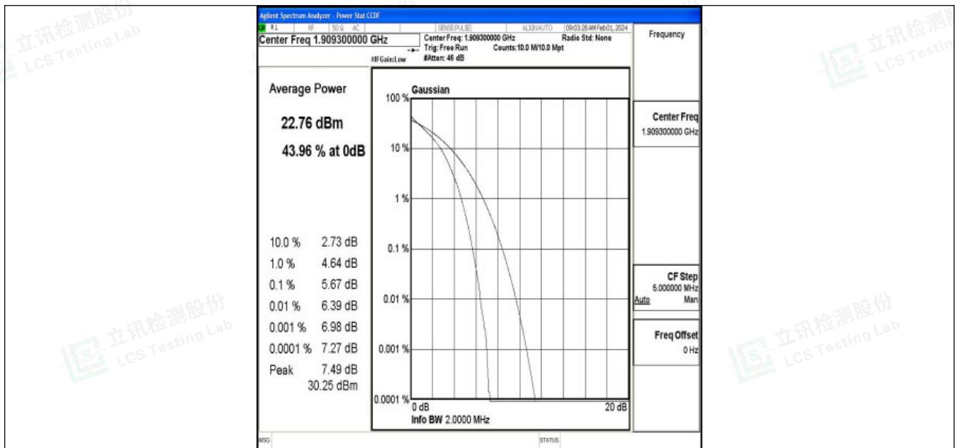
Band2-1.4MHz-QPSK-19193-6RB#0-PASS
