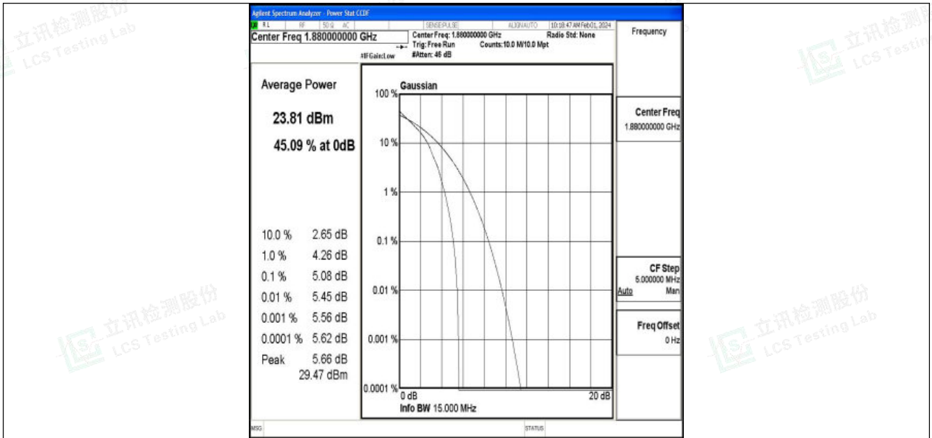
Band2-15MHz-QPSK-18900-1RB#0-PASS
