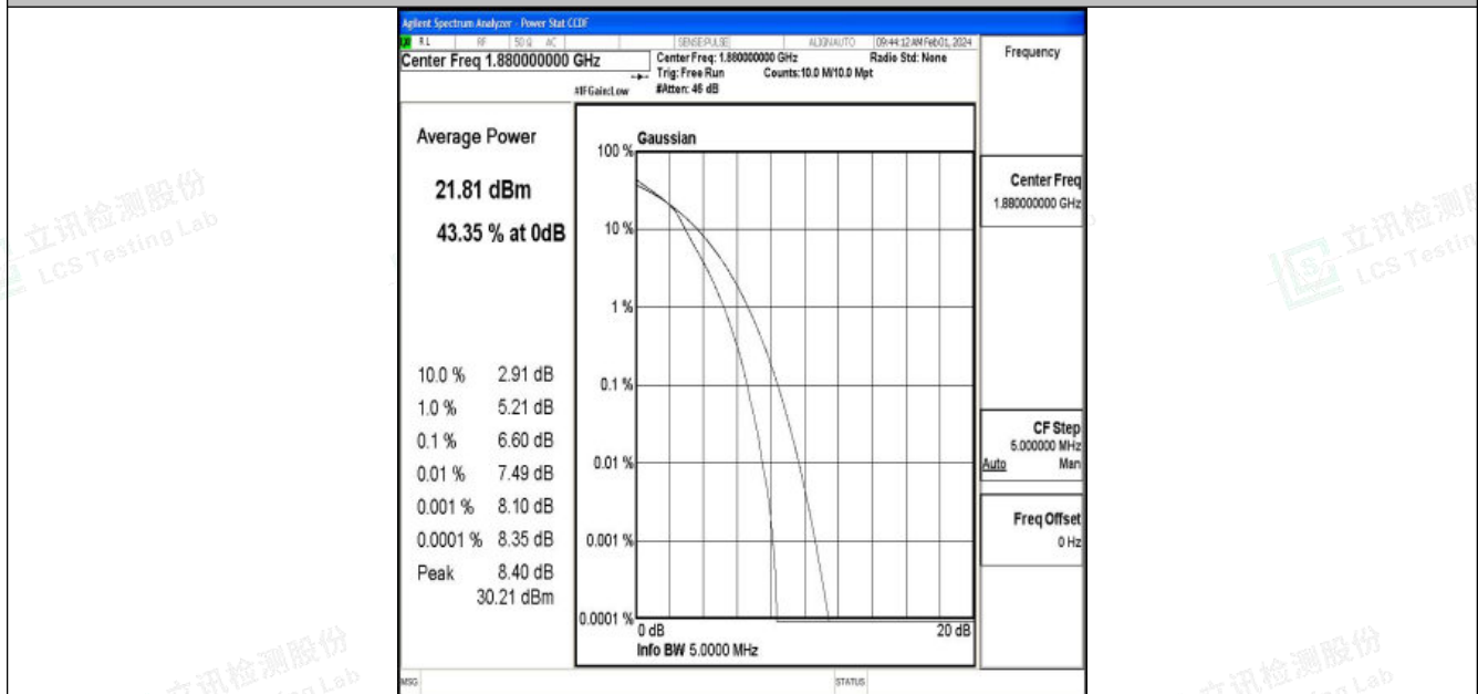
Band2-5MHz-16QAM-18900-25RB#0-PASS
