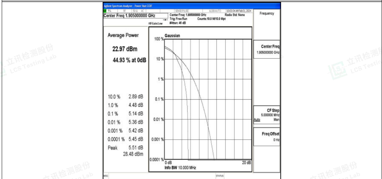
Band2-10MHz-16QAM-19150-1RB#0-PASS
