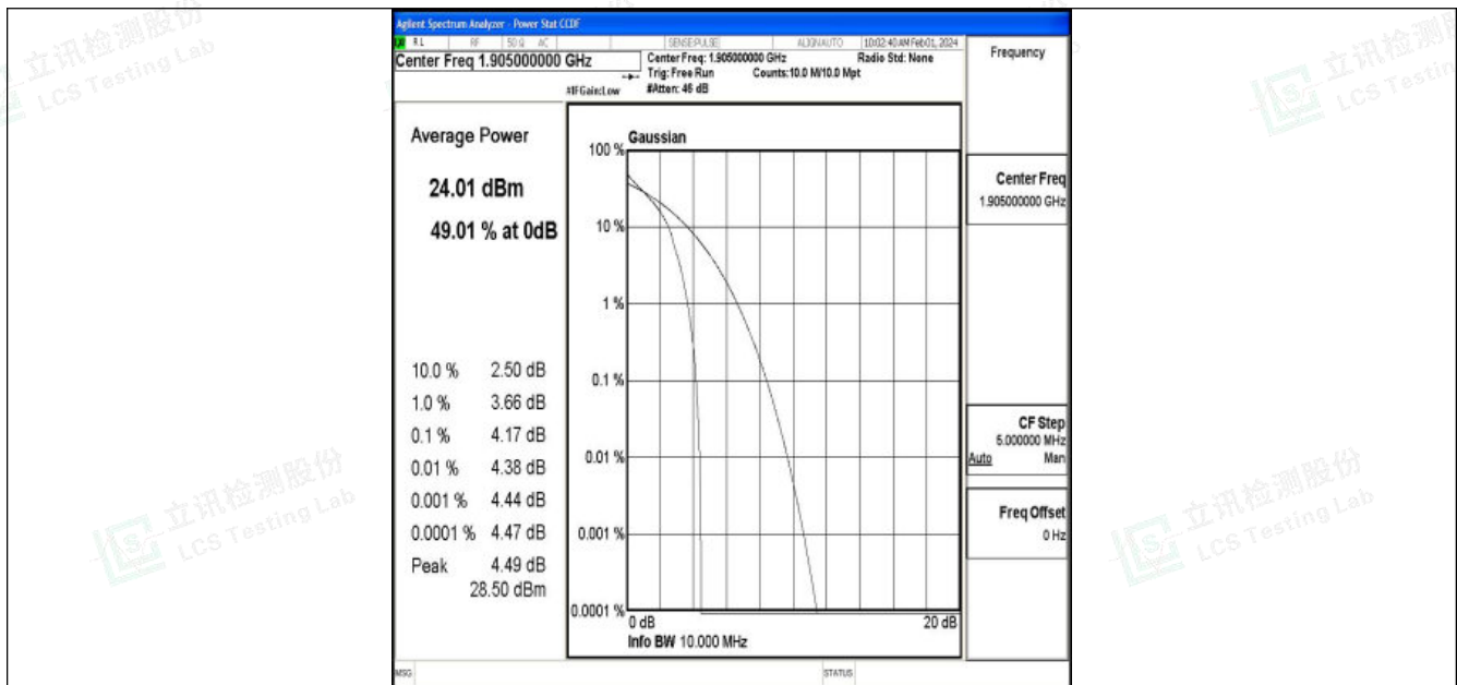
Band2-10MHz-QPSK-19150-1RB#0-PASS
