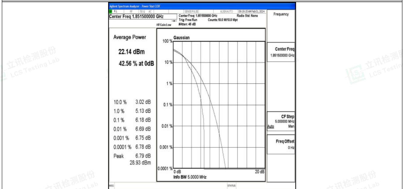
Band2-3MHz-16QAM-18615-1RB#0-PASS
