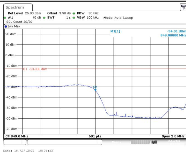
Band5-3MHz-16QAM-20635-1RB#14
