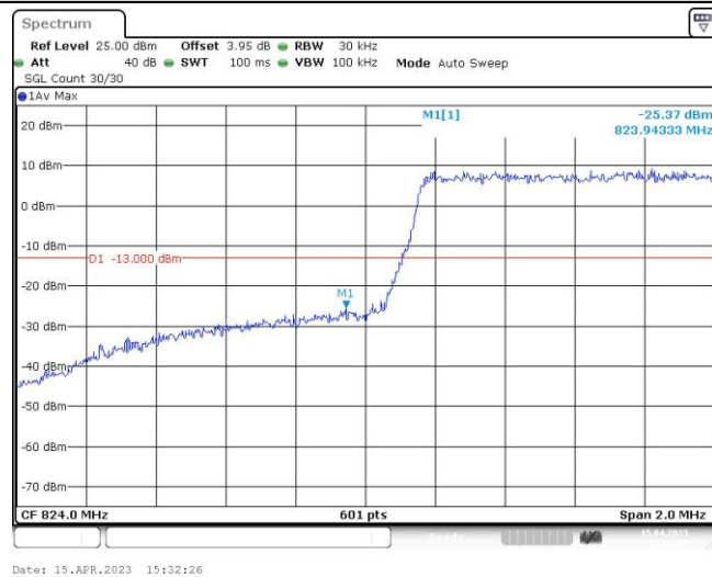
Band5-1.4MHz-16QAM-20643-1RB#0
