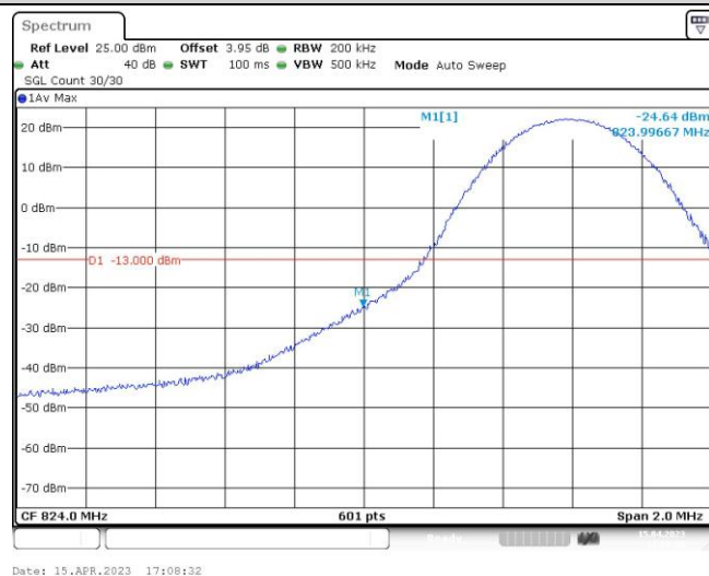
Band5-10MHz-QPSK-20450-1RB#49
