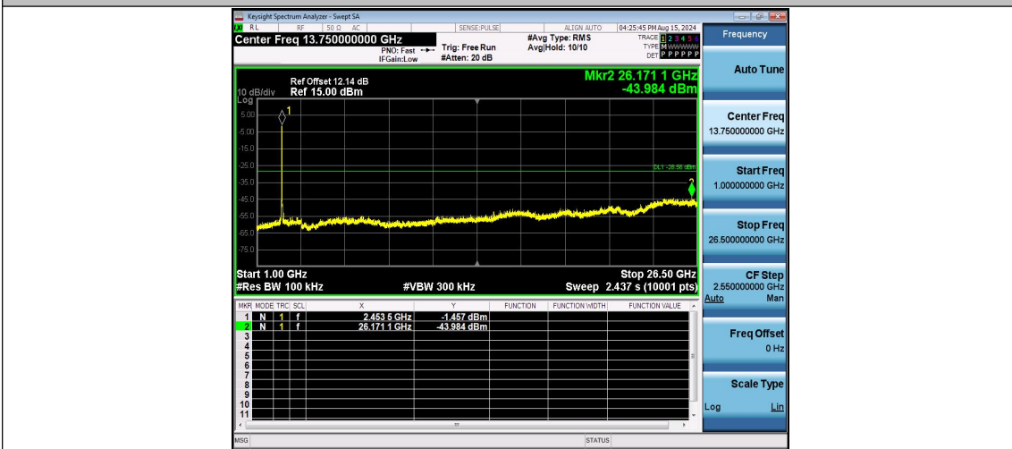
11AX40SISO_Ant0_2452_1000~26500
