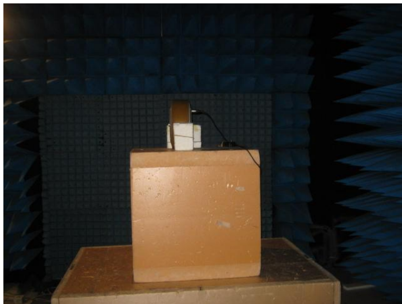
Charging mode
