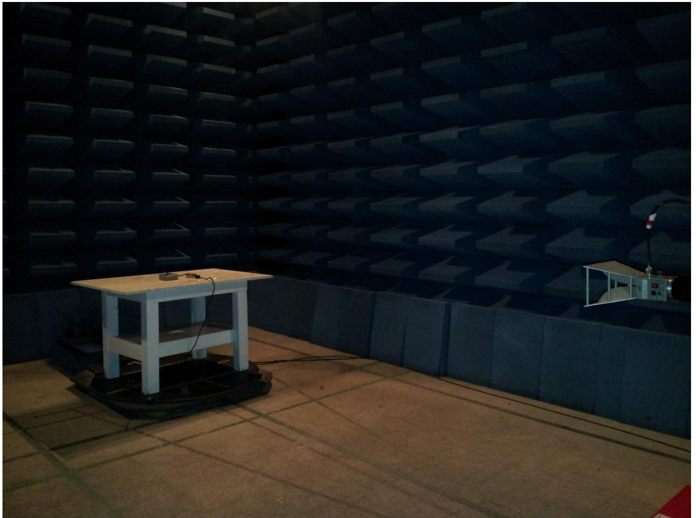
Radiated Emissions Test Setup – Intentional Harmonics(1-10GHz)
