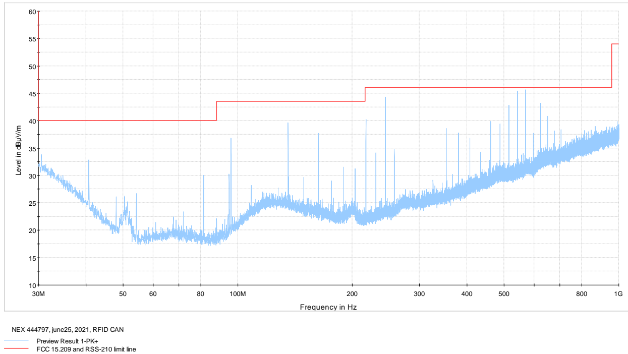
Figure 8.6-2: Field strength of spurious emissions above 30 MHz
