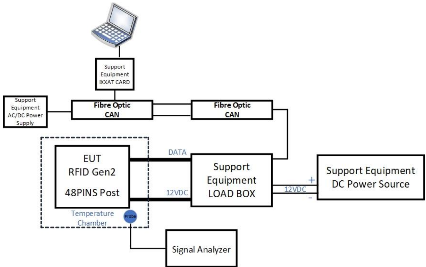
Figure 5.5-2: Antenna port testing block diagram
