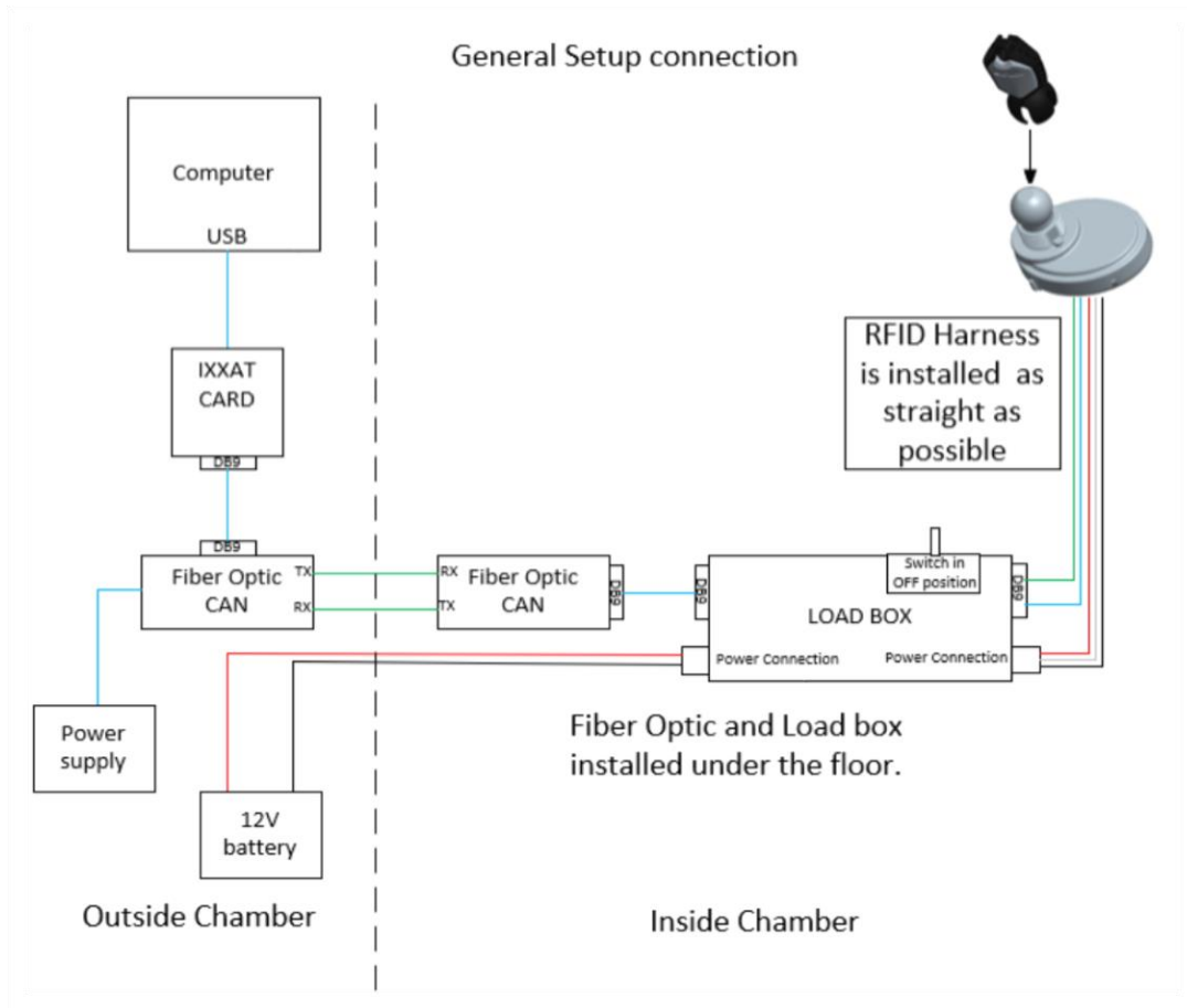
Figure 5.5-1: Radiated testing block diagram
