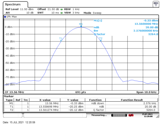
Figure 8.4-2: 20 dB bandwidth
