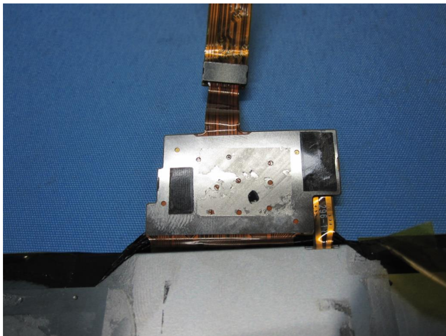
Figure 10 EUT Internal Photo
