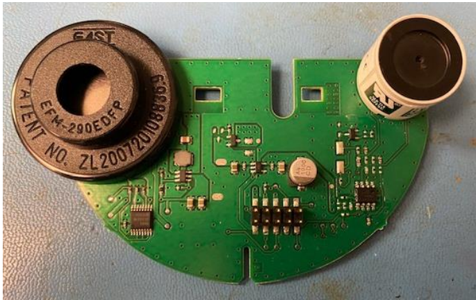
PCB0106 TOP
