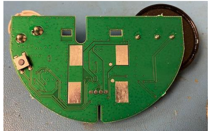
PCB0106 BOTTOM
