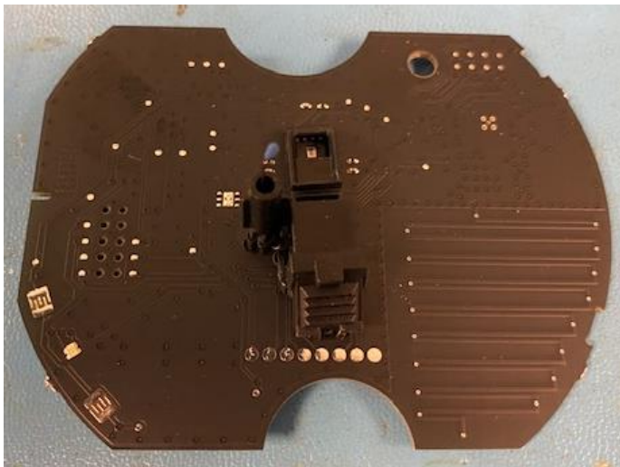
PCB0107 TOP (Only board with Radio)
