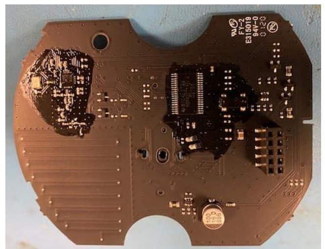
PCB0107 BOTTOM (Only board with Radio)
