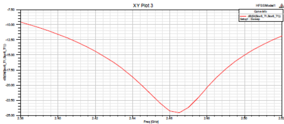
Figure 8. Antenna port S11 simulation curve
