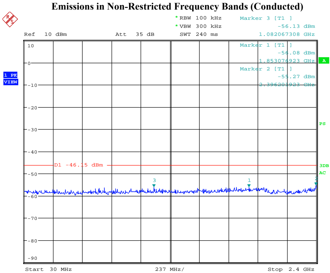
Channel 39 (30 MHz- 2.4 GHz)
