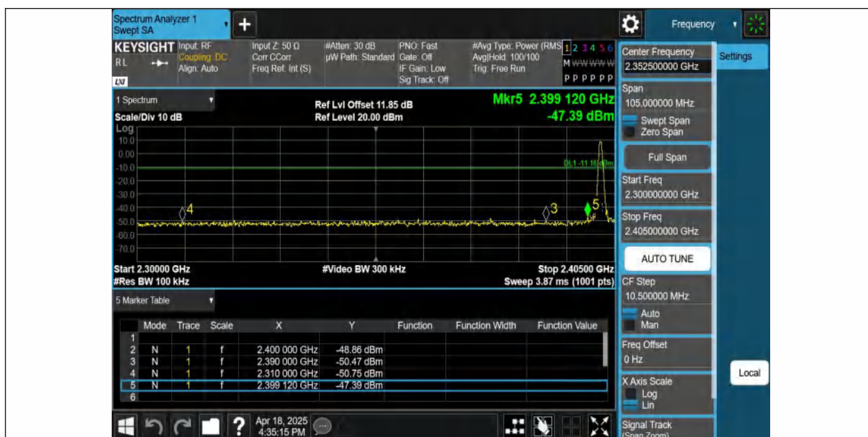
DH5-Ant1-2402-PASS
