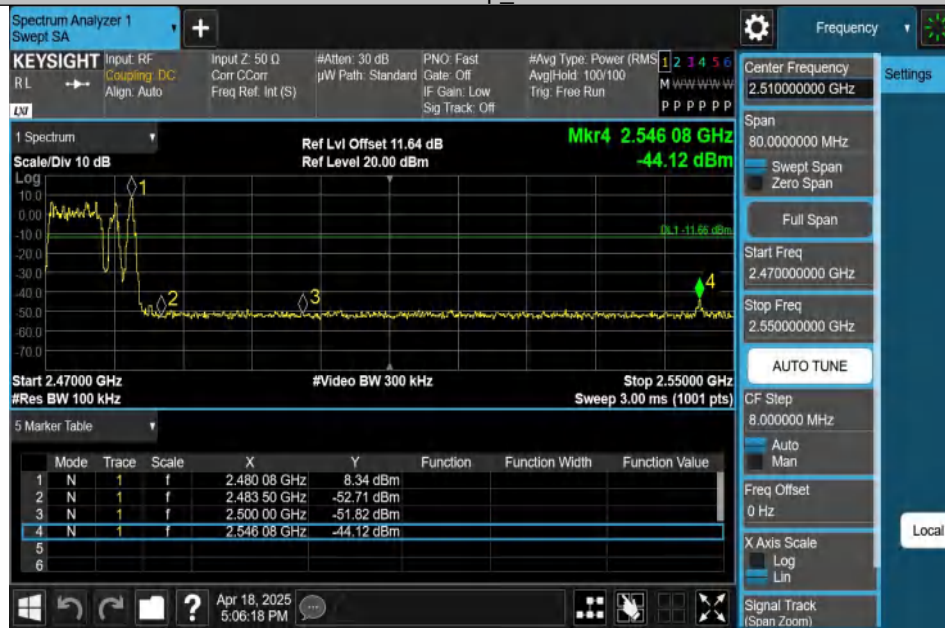
3DH5-Ant1-Hop_2480-PASS
