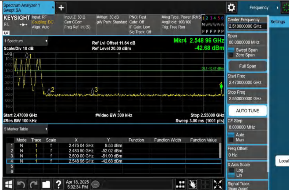
DH5-Ant1-Hop_2480-PASS
