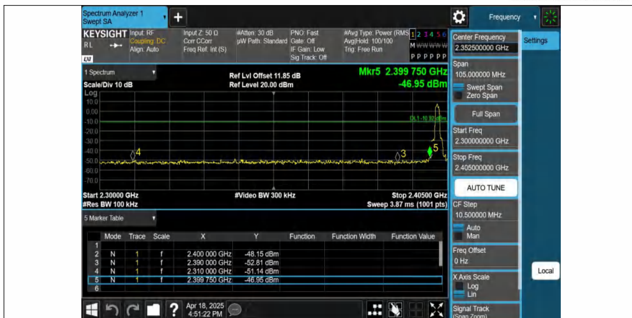
3DH5-Ant1-2402-PASS
