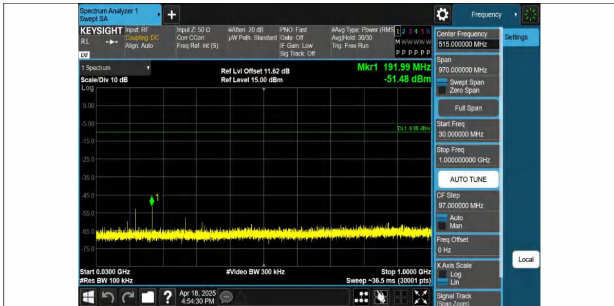
3DH5-Ant1-2441-30~1000-PASS
