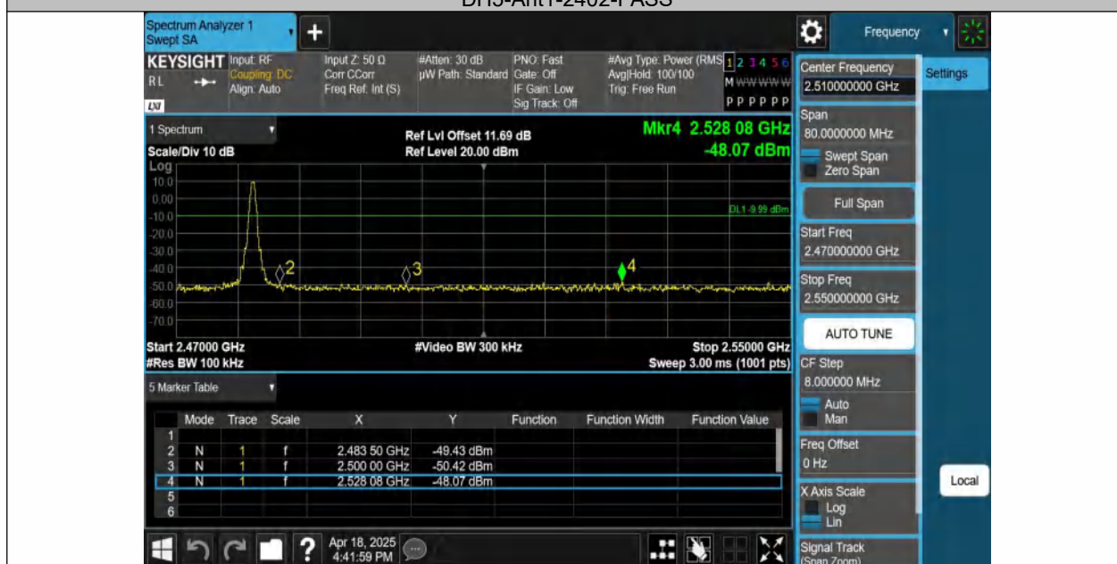
DH5-Ant1-2480-PASS
