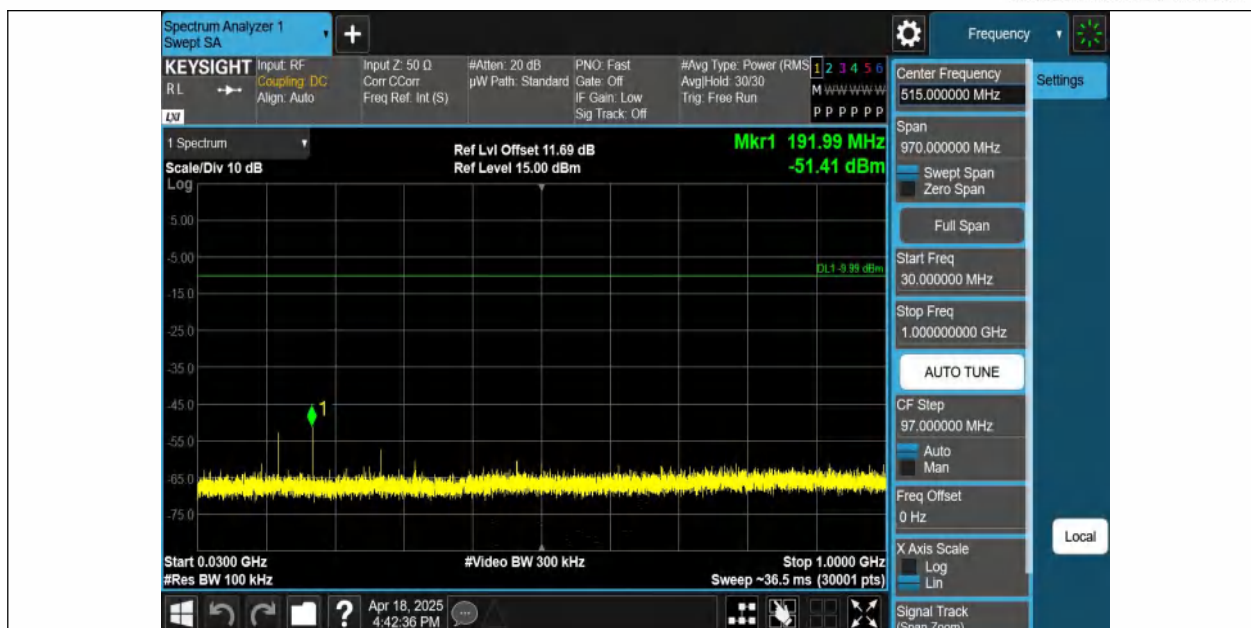
DH5-Ant1-2480-30~1000-PASS
