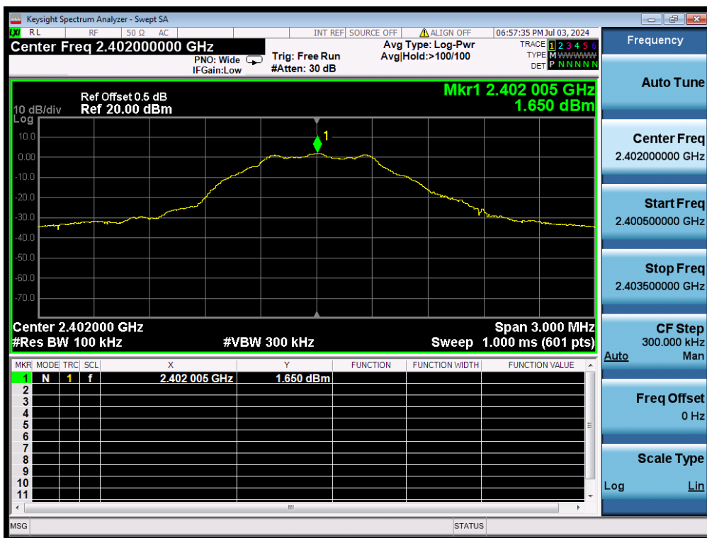
Figure 19: Conducted Spurious Emission & Authorized-band band-edge, 2402MHz, BLE-1Mbps Carrier Level
