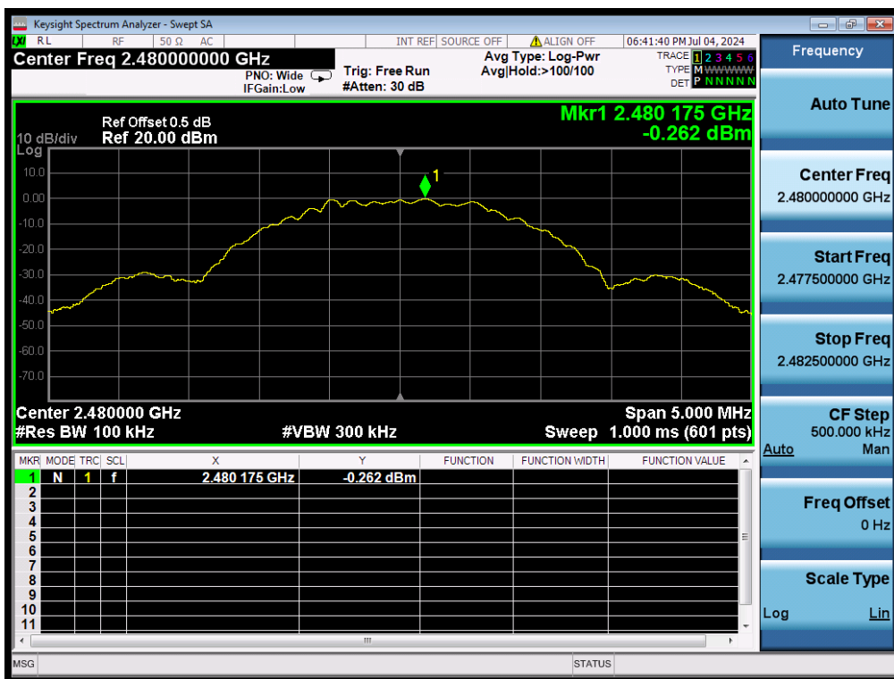
Figure 24: Conducted Spurious Emission & Authorized-band band-edge, 2480MHz, BLE-2Mbps Carrier Level
