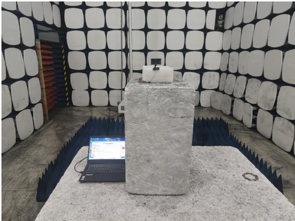
EH-MC26B Model
