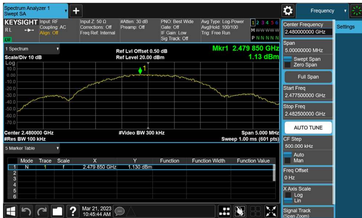
Figure 42: Conducted Spurious Emission & Authorized-band band-edge, 2480MHz, BLE-2M Carrier Level
