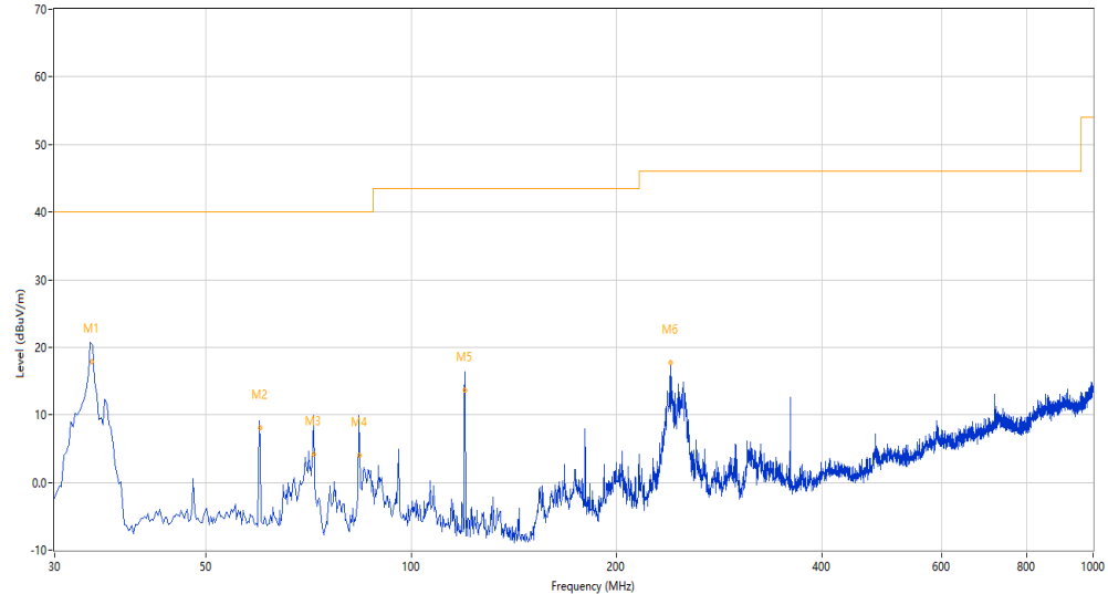
Emission Test case_FCC_Part 15C_FCC 15.247(2.4G)_30MHz-1GHz
