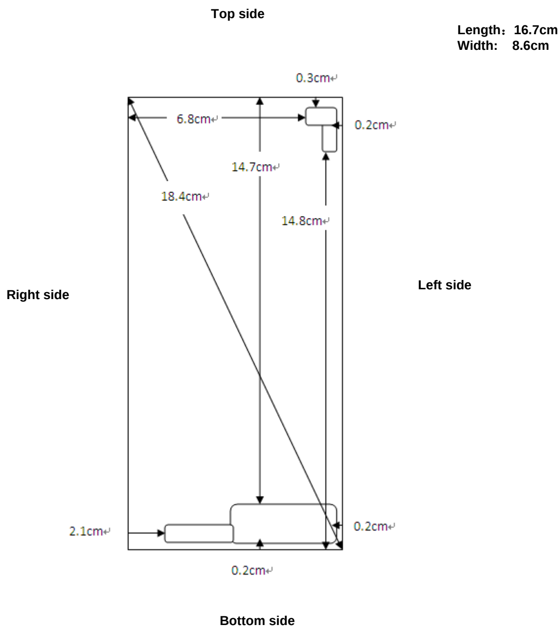
Figure1: The antenna position of the DUT
