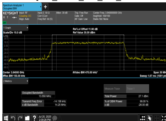
N77(15M)_CP-OFDM_16 QAM_Outer_Full_Mid_CH
