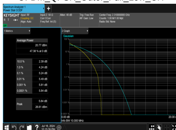
N30(10M)_DFT-s-OFDM QPSK Outer Full Low CH
