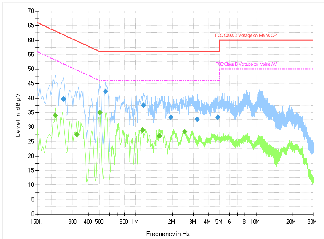
Fig.B.11.1 AC Powerline Conducted Emission- bluetooth
