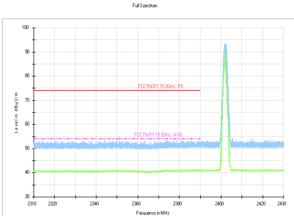
Fig.17. Frequency Band Edges: 8DPSK, Channel 0, 2.31 GHz - 2.43GHz
