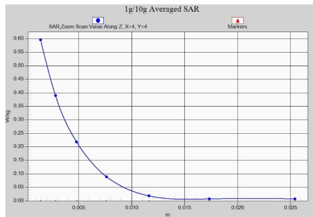
Fig. 1-33 Z-Scan at power reference point (5 GHz)
