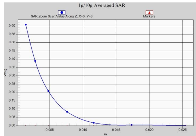
Fig. 1-34 Z-Scan at power reference point (5 GHz)
