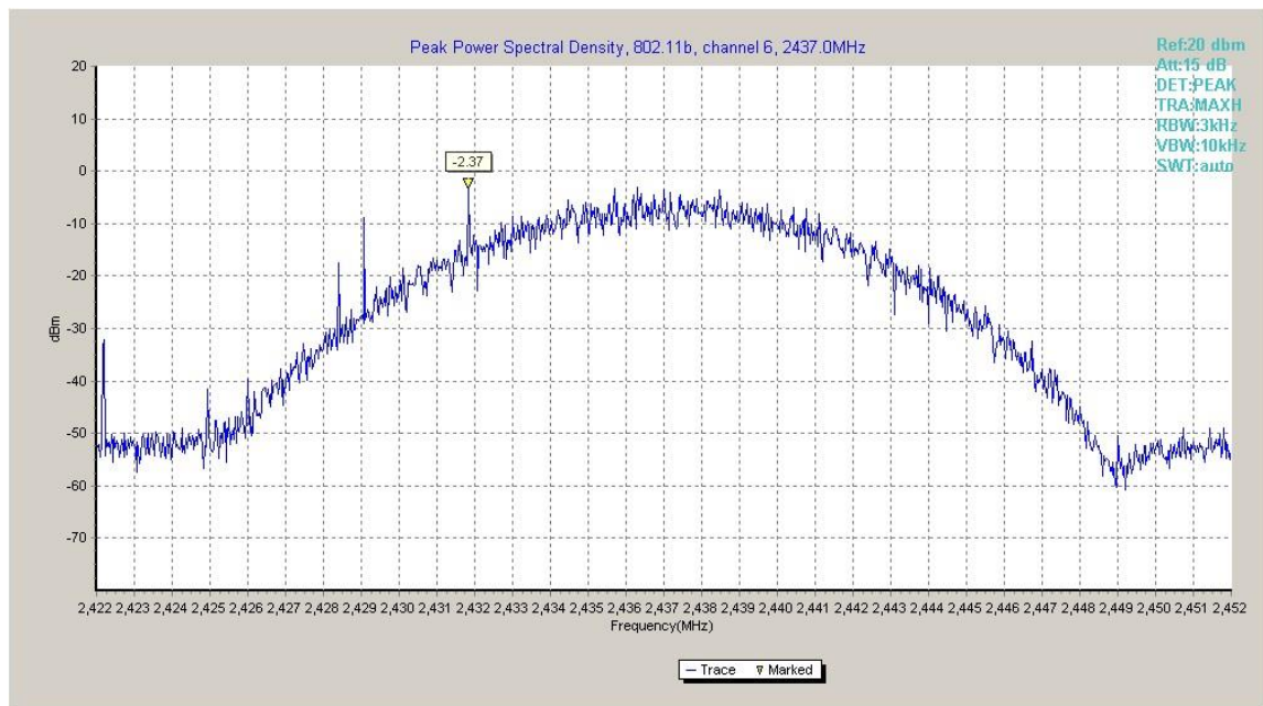
Fig.A.3.2 Power Spectral Density (802.11b, Ch 6)
