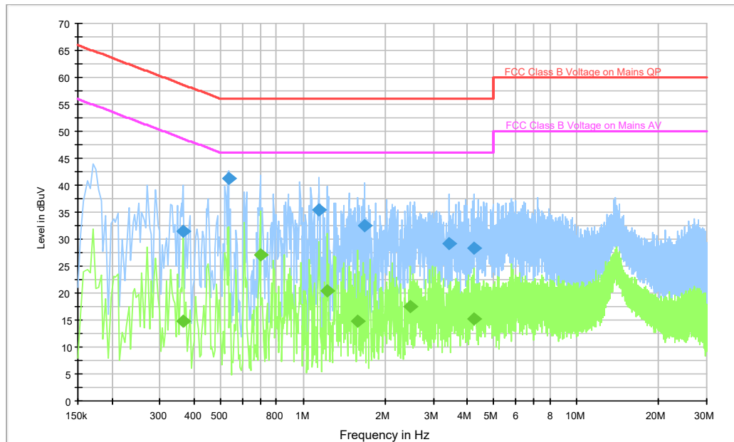
Fig.49 Conducted Emission(802.11a, Ch40, TX, With charger QC16US)
