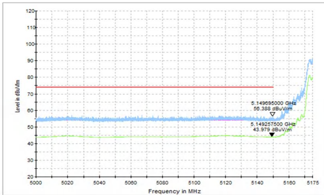
Fig. 9 Band Edges (802.11n-HT40 Ch38, 5190MHz, FULL RU)
