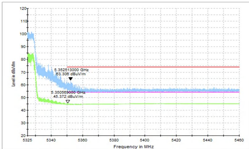
Fig. 42 Band Edges (802.11ax-HT40 Ch62, 5310MHz, PARTIAL RU)
