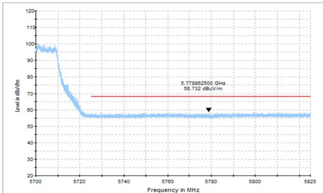
Fig. 28 Band Edges (802.11ax-HT20 Ch140, 5700MHz, FULL RU)
