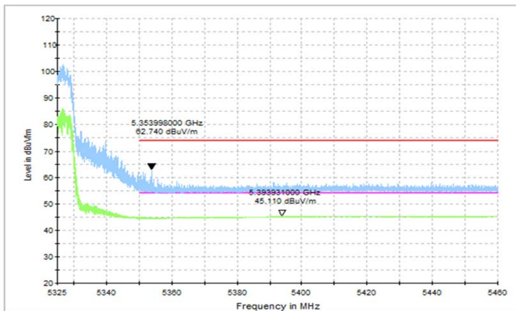
Fig. 46 Band Edges (802.11ax-HT80 Ch58, 5290MHz), PARTIAL RU
