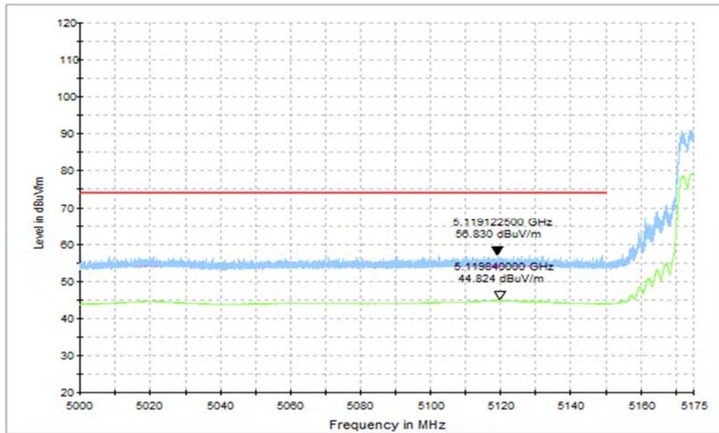
Fig. 29 Band Edges (802.11ax-HT40 Ch38, 5190MHz, FULL RU)
