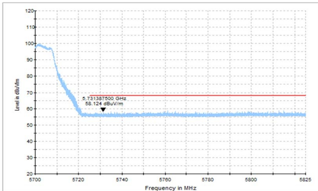
Fig. 4 Band Edges (802.11a Ch140, 5700MHz, FULL RU)
