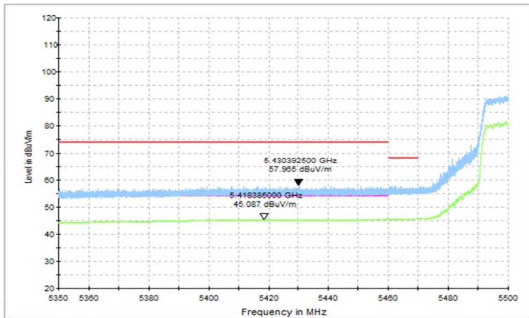
Fig. 19 Band Edges (802.11ac-HT40 Ch102, 5510MHz, FULL RU)
