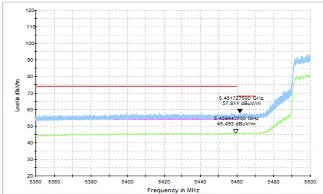
Fig. 31 Band Edges (802.11ax-HT40 Ch102, 5510MHz, FULL RU)
