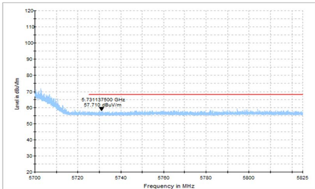
Fig. 12 Band Edges (802.11n-HT40 Ch134, 5670MHz, FULL RU)
