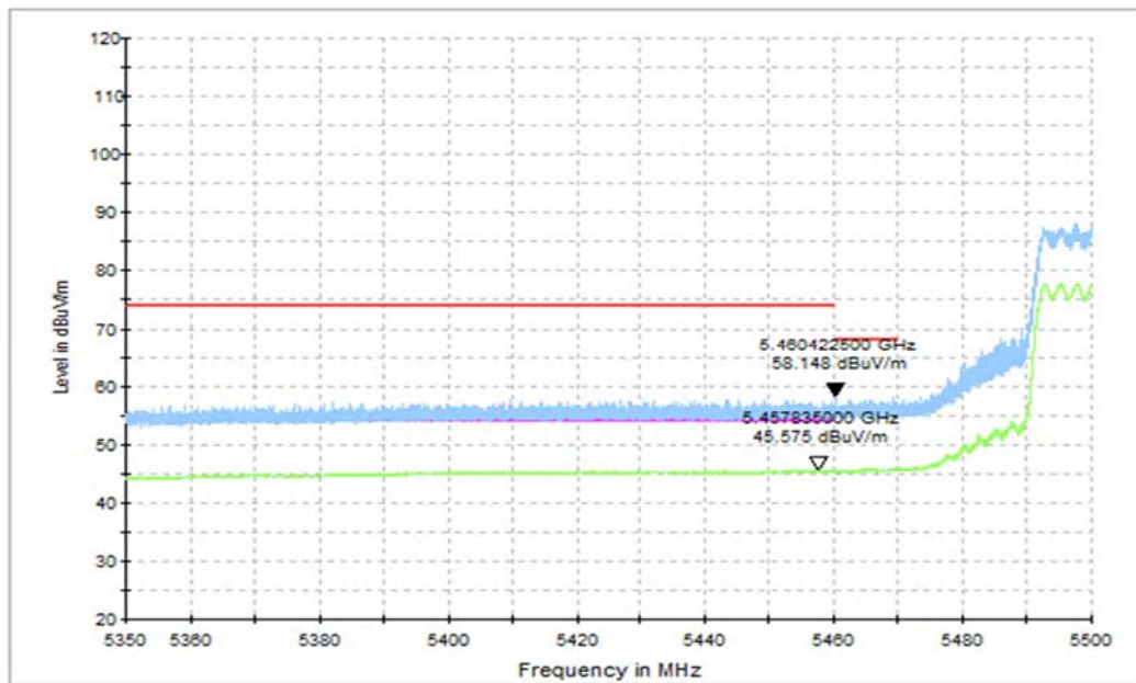
Fig. 23 Band Edges (802.11ac-HT80 Ch106, 5530MHz, FULL RU)
