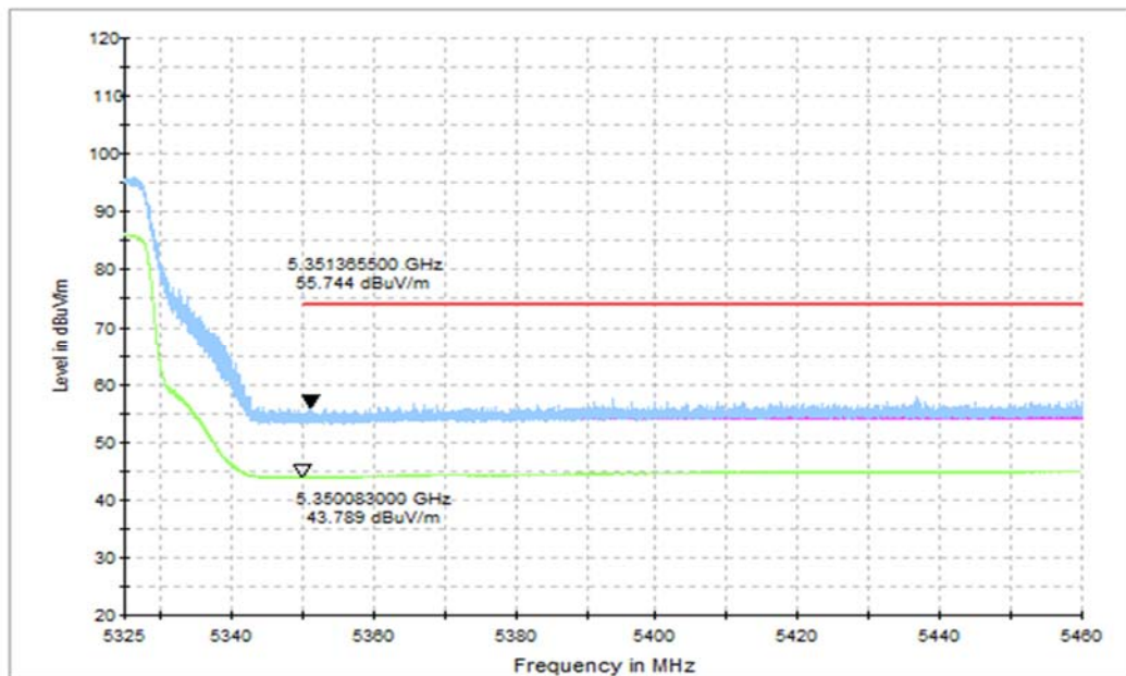
Fig. 2 Band Edges (802.11a Ch64, 5320MHz, FULL RU)
