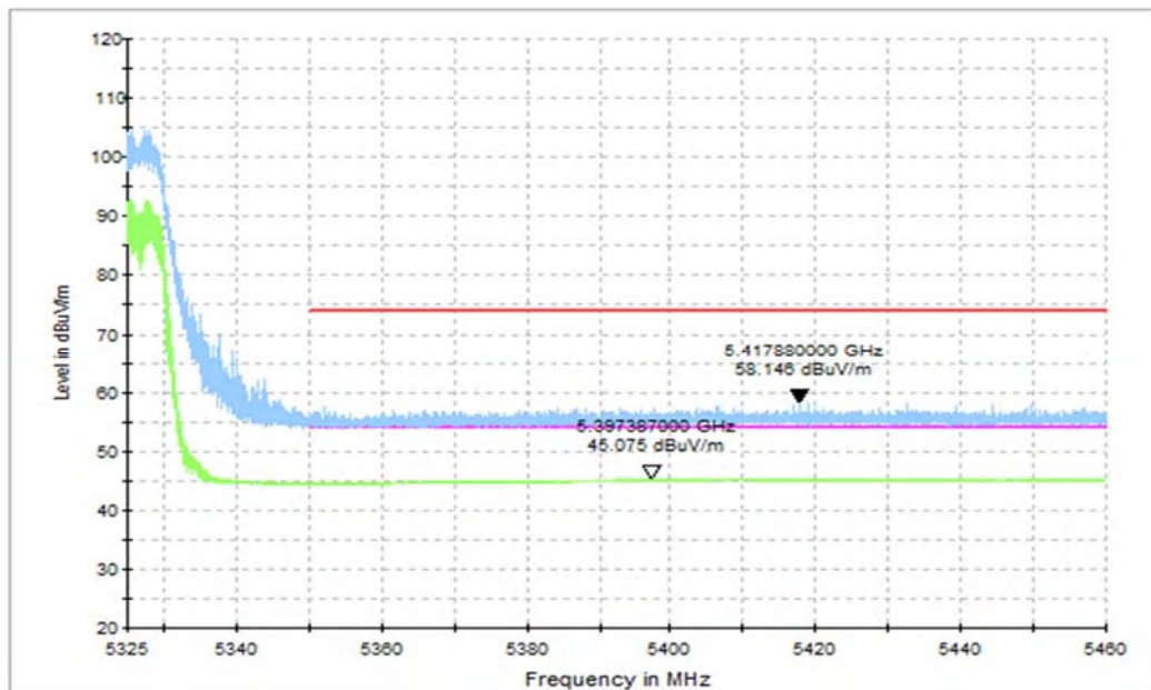
Fig. 38 Band Edges (802.11ax-HT20 Ch64, 5320MHz, PARTIAL RU)
