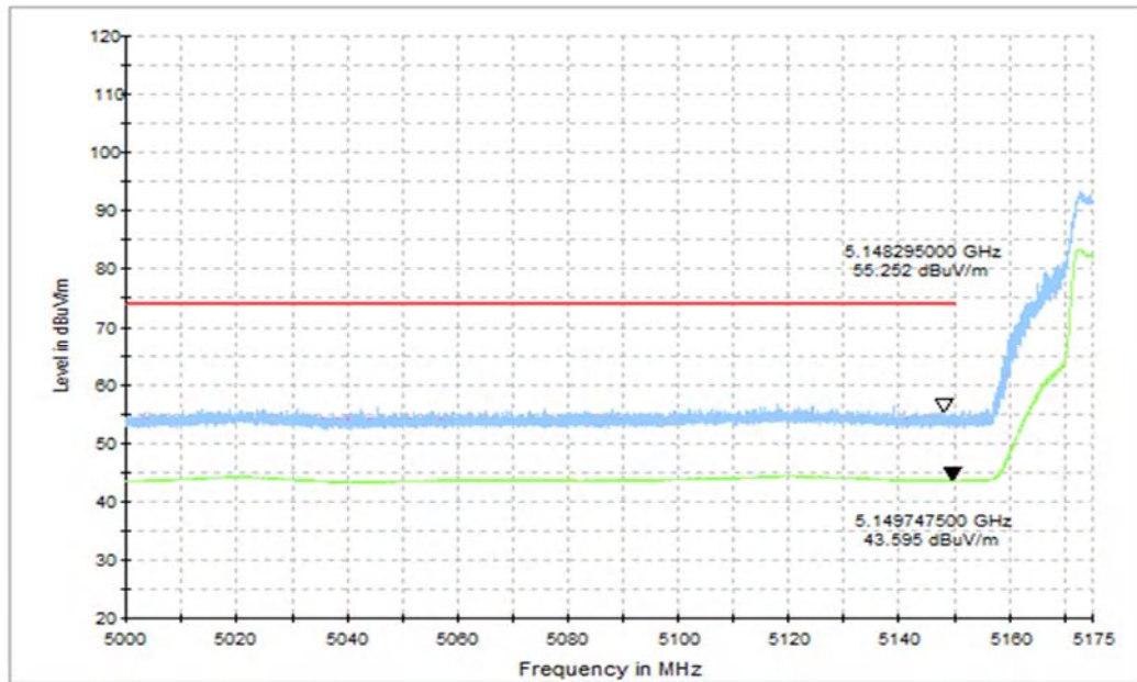
Fig. 1 Band Edges (802.11a Ch36, 5180MHz, FULL RU)
