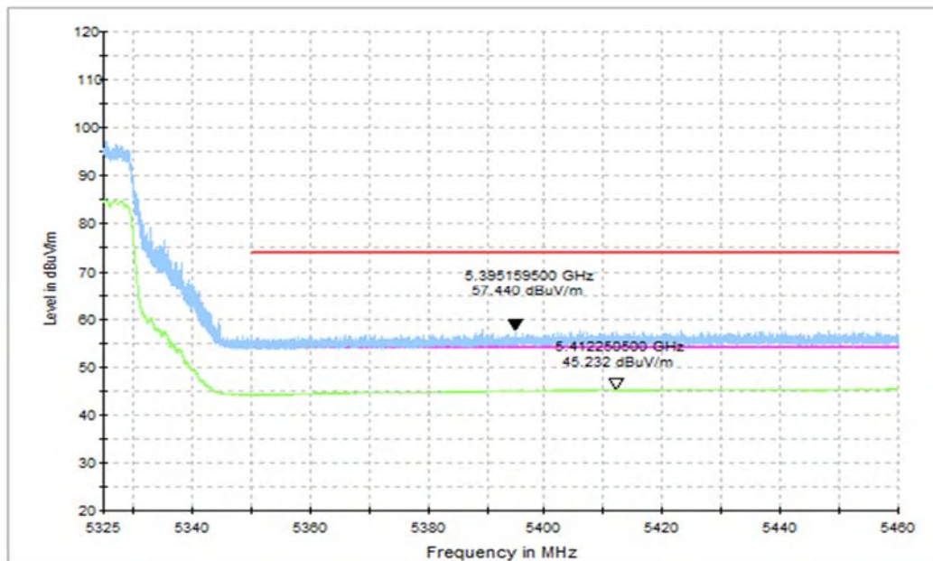
Fig. 26 Band Edges (802.11ax-HT20 Ch64, 5320MHz, FULL RU)
