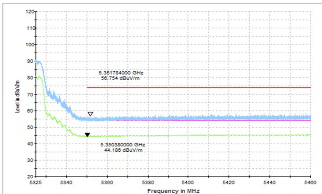
Fig. 10 Band Edges (802.11n-HT40 Ch62, 5310MHz, FULL RU)
