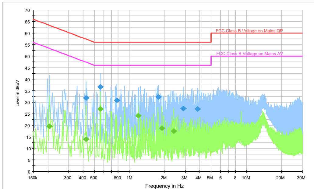
Fig.50 Conducted Emission(802.11a, IDLE, With charger QC16US)
