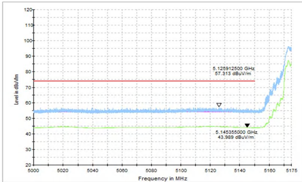
Fig. 13 Band Edges (802.11ac-HT20 Ch36, 5180MHz, FULL RU)
