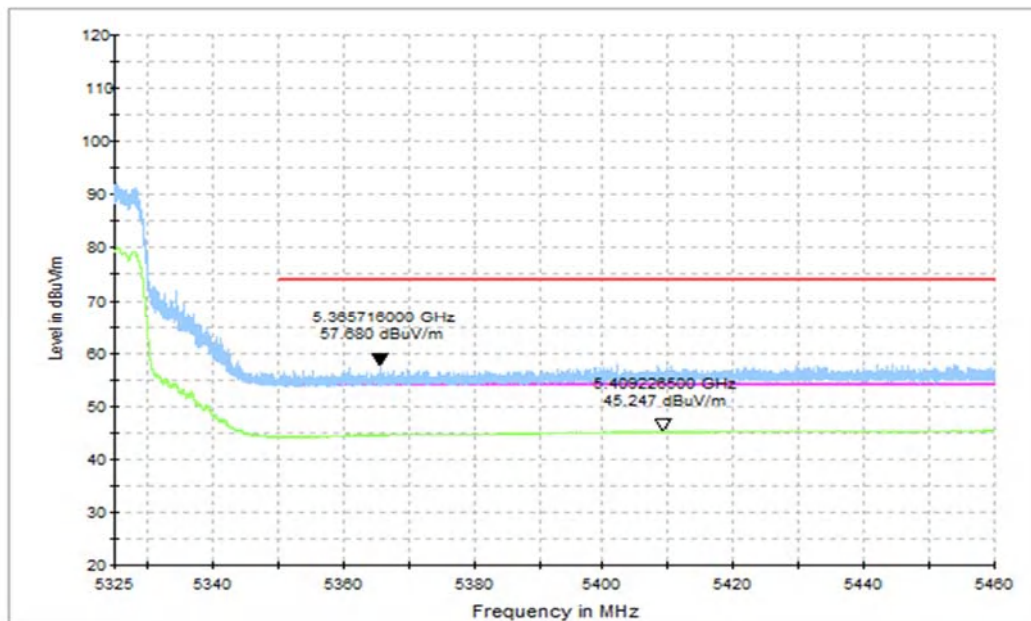
Fig. 30 Band Edges (802.11ax-HT40 Ch62, 5310MHz, FULL RU)
