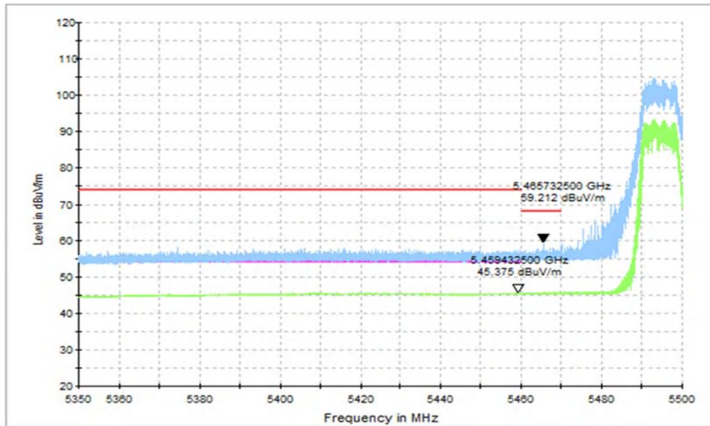
Fig. 39 Band Edges (802.11ax-HT20 Ch100, 5500MHz, PARTIAL RU)
