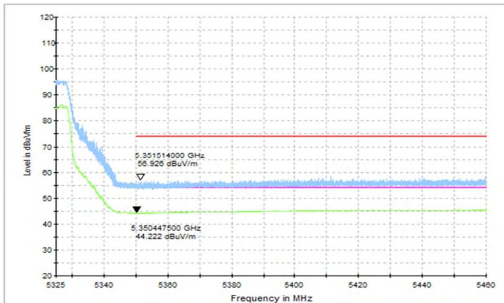
Fig. 14 Band Edges (802.11ac-HT20 Ch64, 5320MHz, FULL RU)
