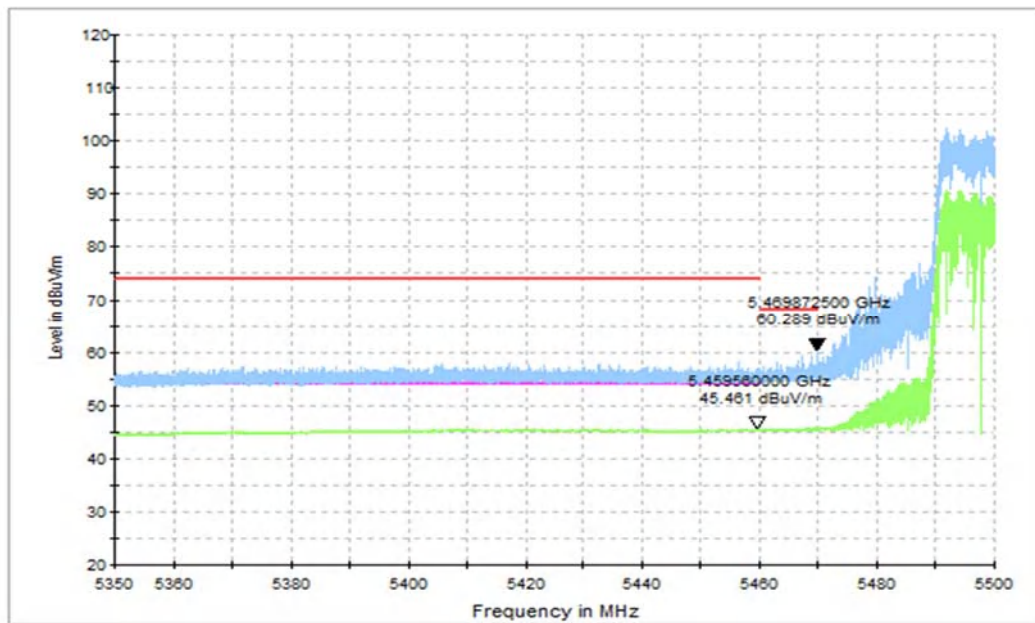
Fig. 47 Band Edges (802.11ax-HT80 Ch106, 5530MHz, PARTIAL RU)
