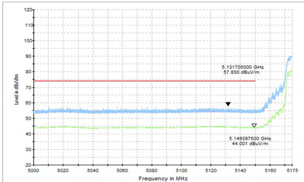
Fig. 17 Band Edges (802.11ac-HT40 Ch38, 5190MHz, FULL RU)
