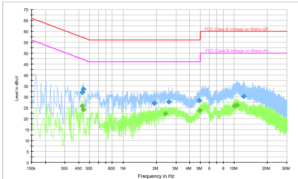
Fig.51 AC Powerline Conducted Emission-802.11a With charger QC16EU
