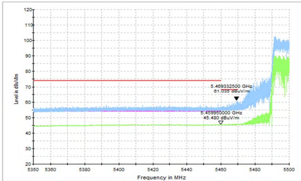
Fig. 43 Band Edges (802.11ax-HT40 Ch102, 5510MHz, PARTIAL RU)
