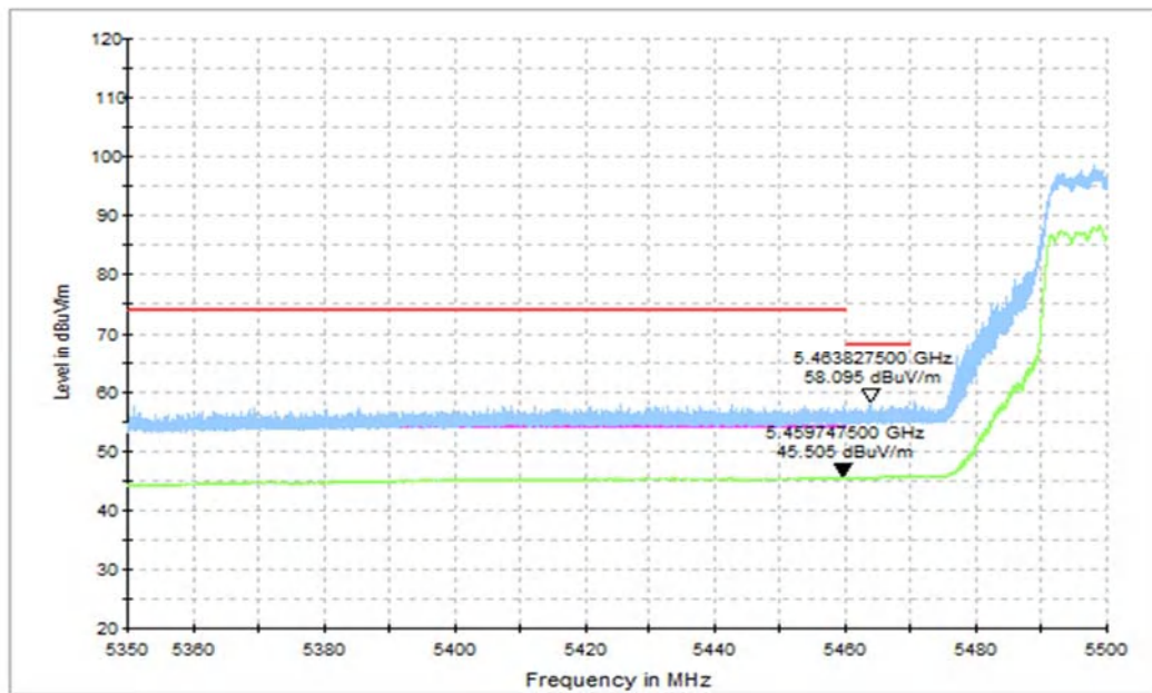
Fig. 7 Band Edges (802.11n-HT20 Ch100, 5500MHz, FULL RU)
