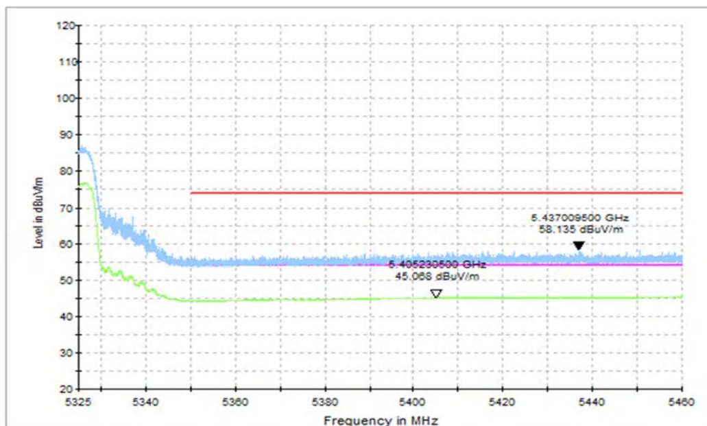
Fig. 22 Band Edges (802.11ac-HT80 Ch58, 5290MHz), FULL RU
