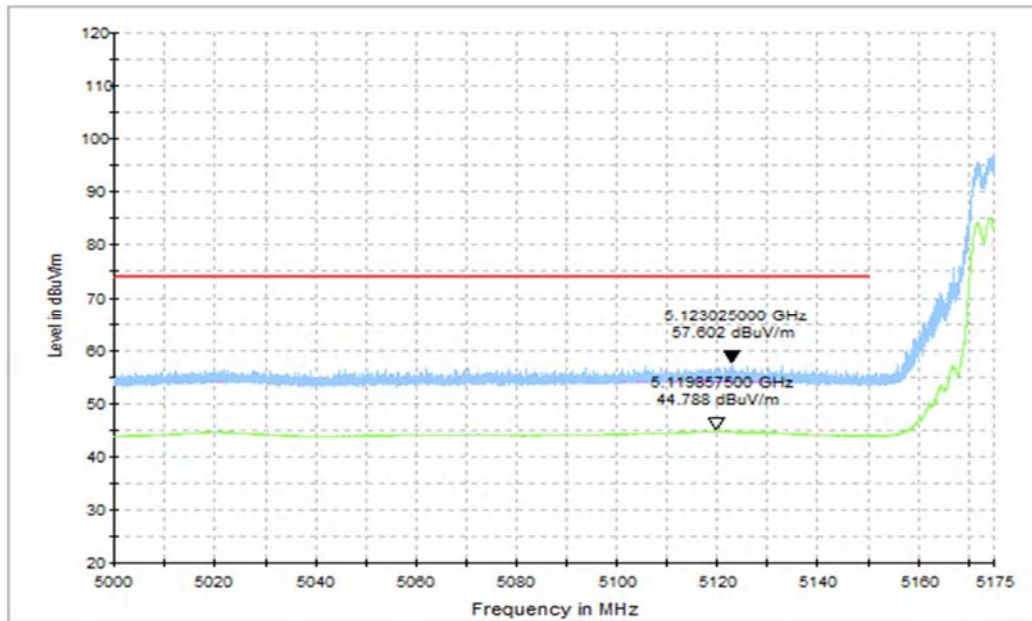
Fig. 25 Band Edges (802.11ax-HT20 Ch36, 5180MHz, FULL RU)
