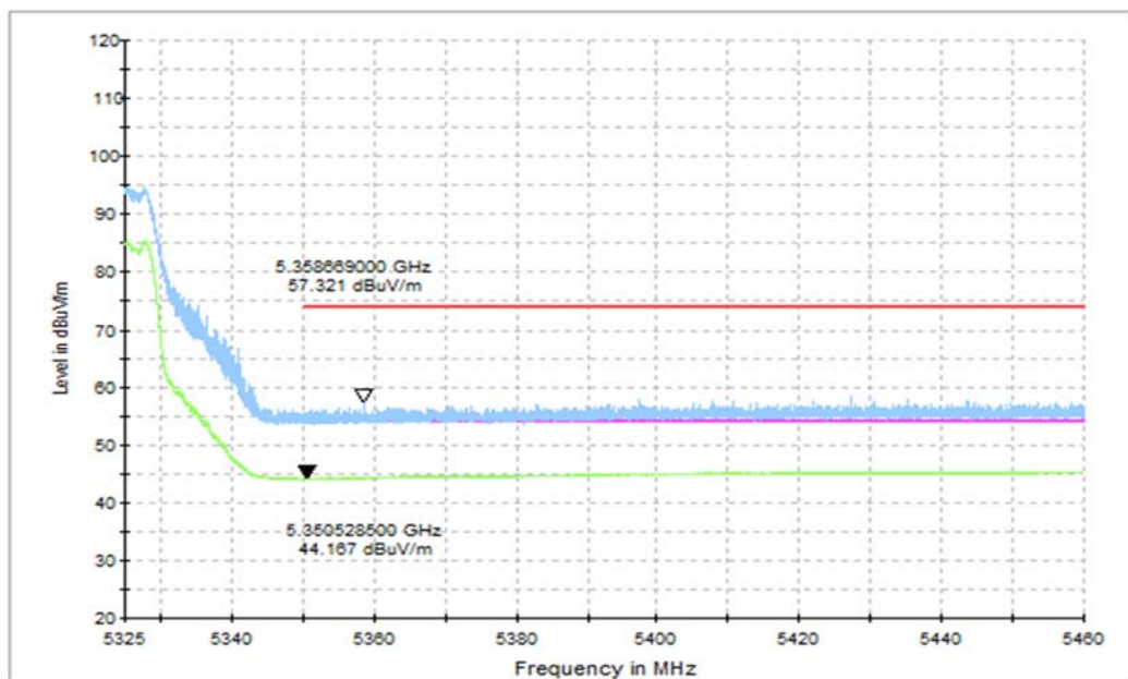
Fig. 6 Band Edges (802.11n-HT20 Ch64, 5320MHz, FULL RU)
