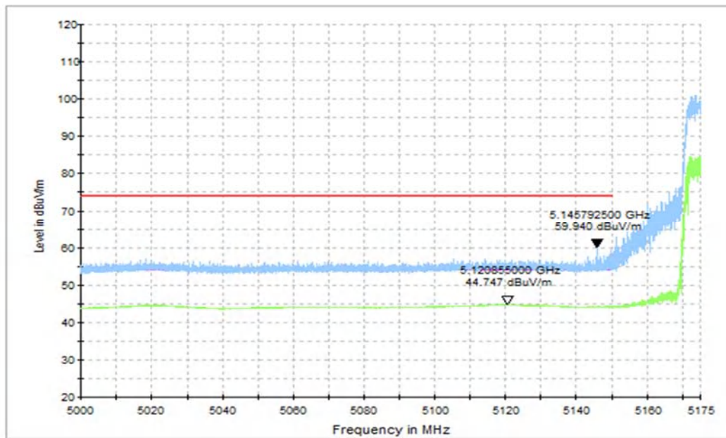
Fig. 45 Band Edges (802.11ax-HT80 Ch42 , 5210MHz, PARTIAL RU)
