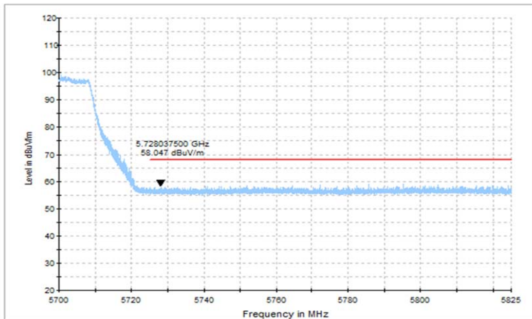
Fig. 16 Band Edges (802.11ac-HT20 Ch140, 5700MHz, FULL RU)
