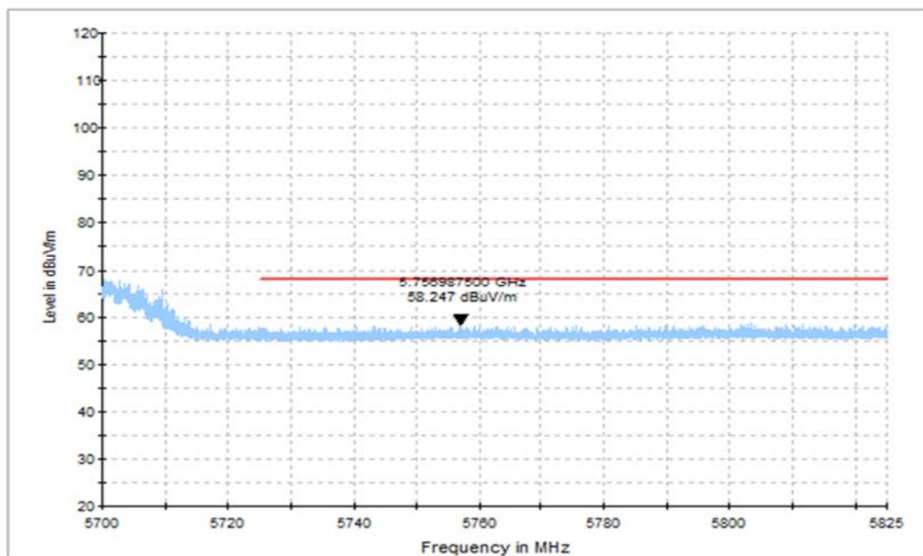
Fig. 20 Band Edges (802.11ac-HT40 Ch134, 5670MHz, FULL RU)
