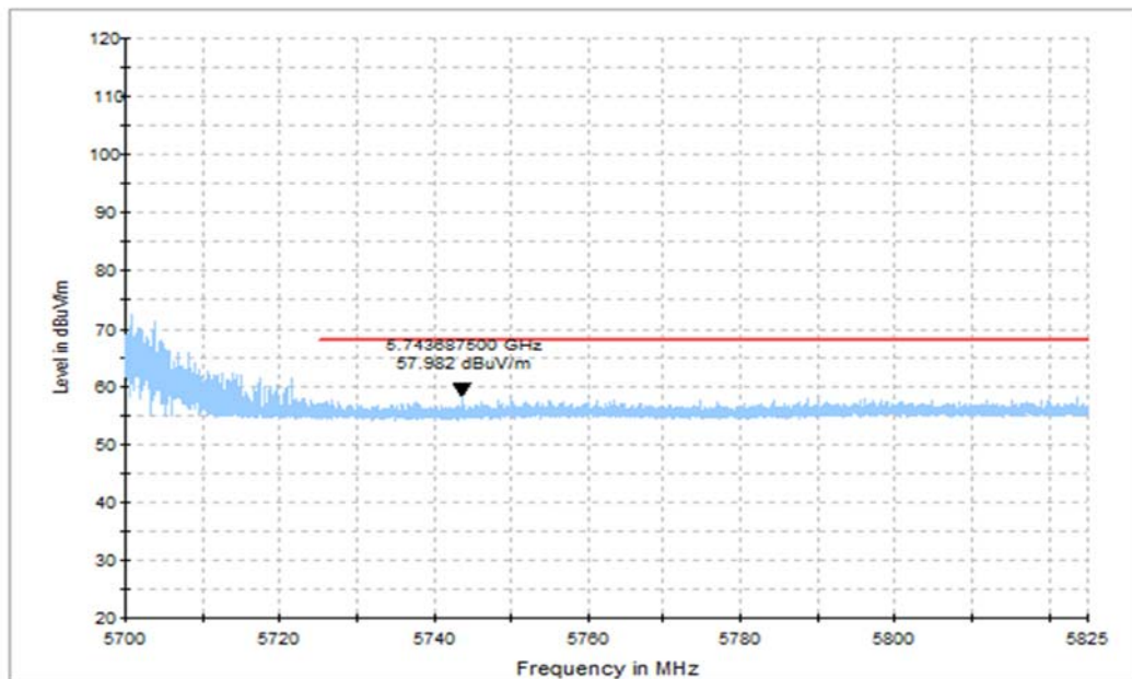
Fig. 44 Band Edges (802.11ax-HT40 Ch134, 5670MHz, PARTIAL RU)
