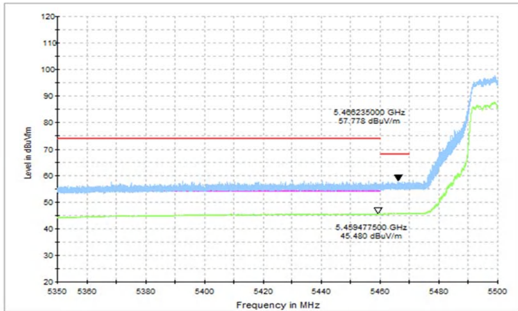
Fig. 15 Band Edges (802.11ac-HT20 Ch100, 5500MHz, FULL RU)
