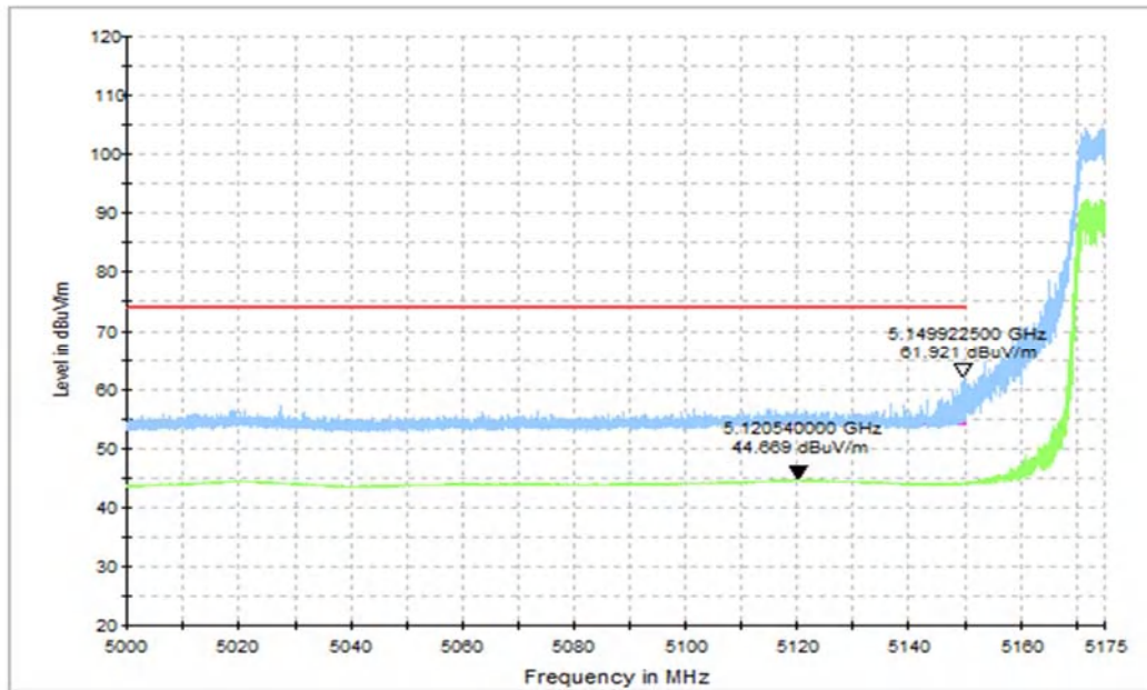
Fig. 37 Band Edges (802.11ax-HT20 Ch36, 5180MHz, PARTIAL RU)
