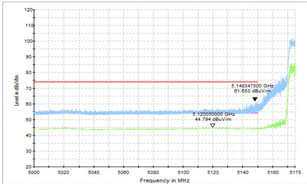
Fig. 41 Band Edges (802.11ax-HT40 Ch38, 5190MHz, PARTIAL RU)
