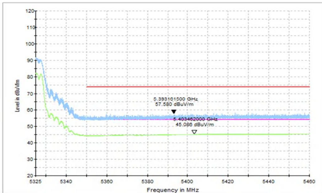
Fig. 18 Band Edges (802.11ac-HT40 Ch62, 5310MHz, FULL RU)
