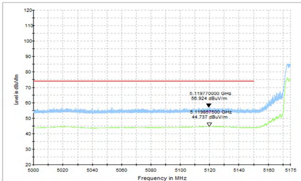
Fig. 21 Band Edges (802.11ac-HT80 Ch42 , 5210MHz, FULL RU)
