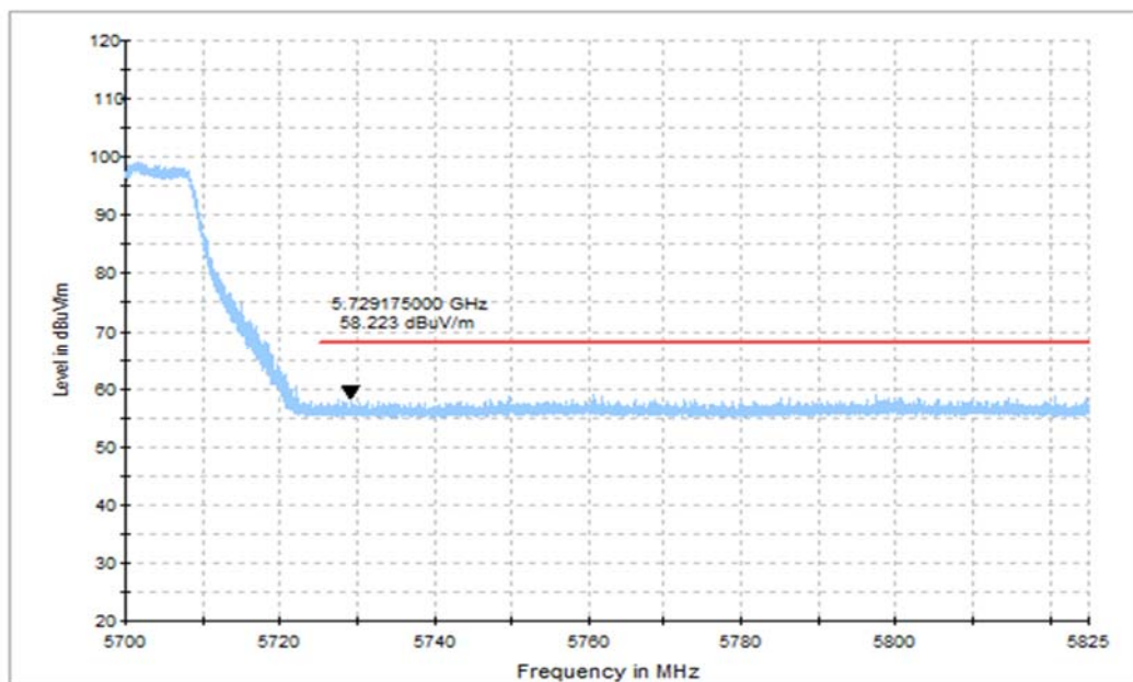
Fig. 8 Band Edges (802.11n-HT20 Ch140, 5700MHz, FULL RU)
