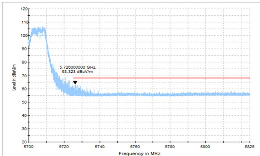
Fig. 40 Band Edges (802.11ax-HT20 Ch140, 5700MHz, PARTIAL RU)
