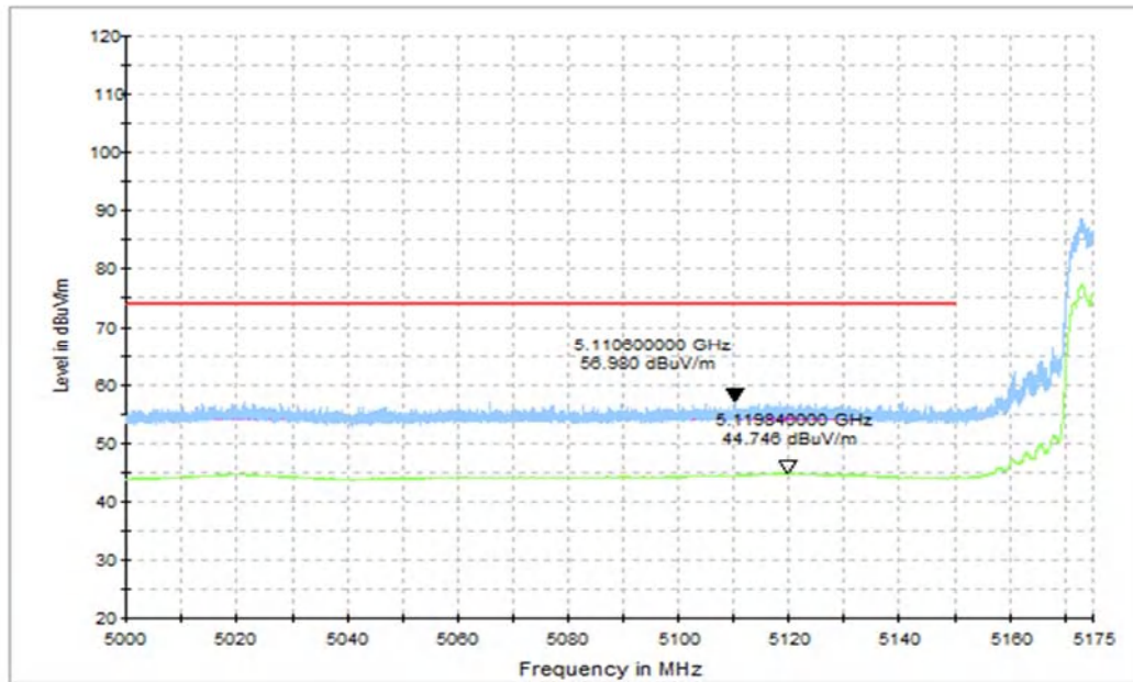
Fig. 33 Band Edges (802.11ax-HT80 Ch42 , 5210MHz, FULL RU)
