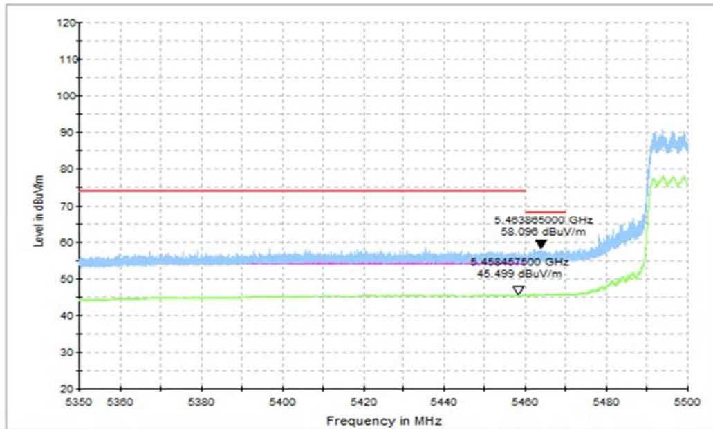
Fig. 35 Band Edges (802.11ax-HT80 Ch106, 5530MHz, FULL RU)
