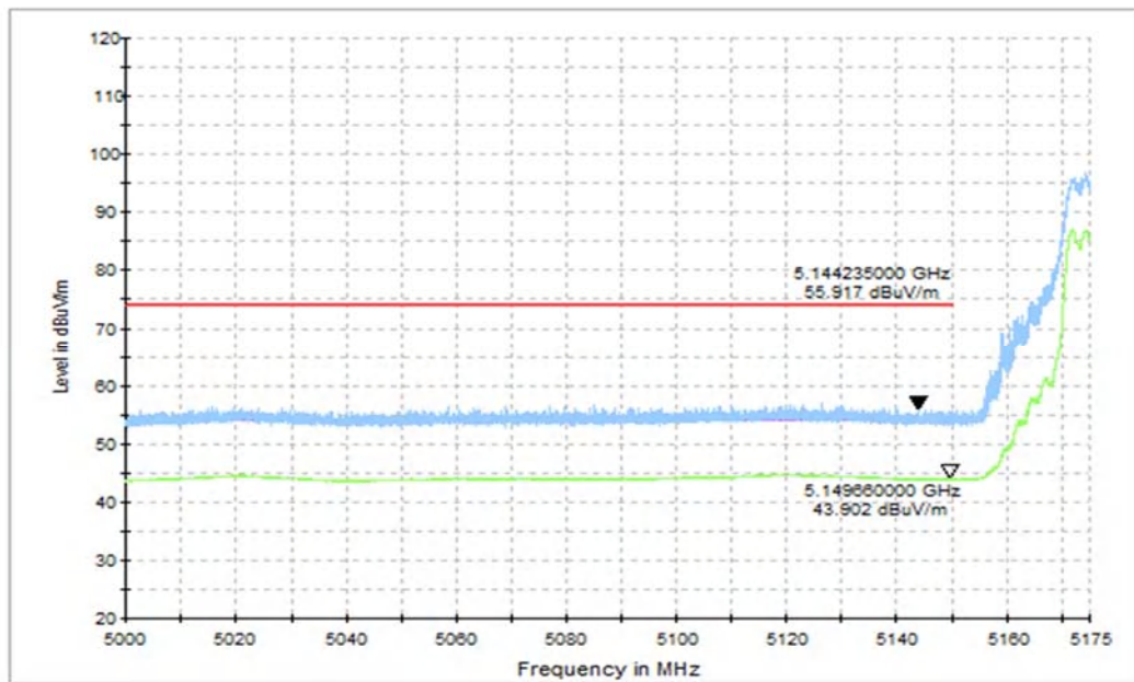
Fig. 5 Band Edges (802.11n-HT20 Ch36, 5180MHz, FULL RU)
