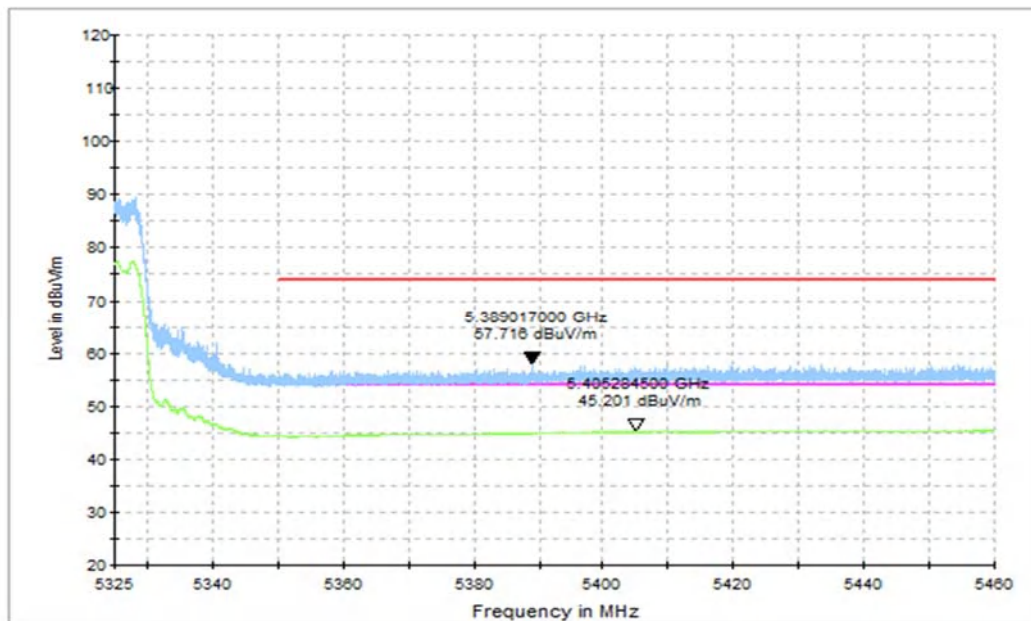
Fig. 34 Band Edges (802.11ax-HT80 Ch58, 5290MHz) , FULL RU
