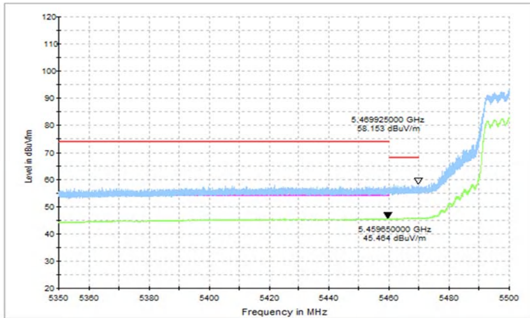
Fig. 11 Band Edges (802.11n-HT40 Ch102, 5510MHz, FULL RU)
