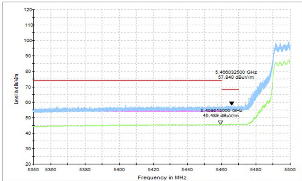
Fig. 27 Band Edges (802.11ax-HT20 Ch100, 5500MHz, FULL RU)
