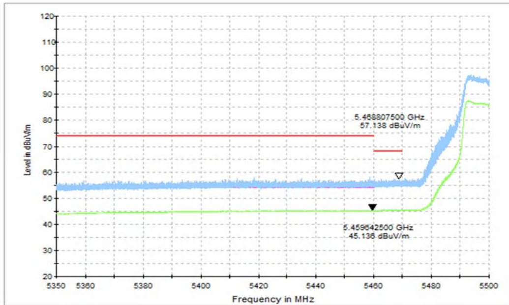
Fig. 3 Band Edges (802.11a Ch100, 5500MHz, FULL RU)
