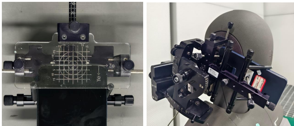
Pic 3: Handset Positioner (HHPIII) with mounted EUT mobile phone
