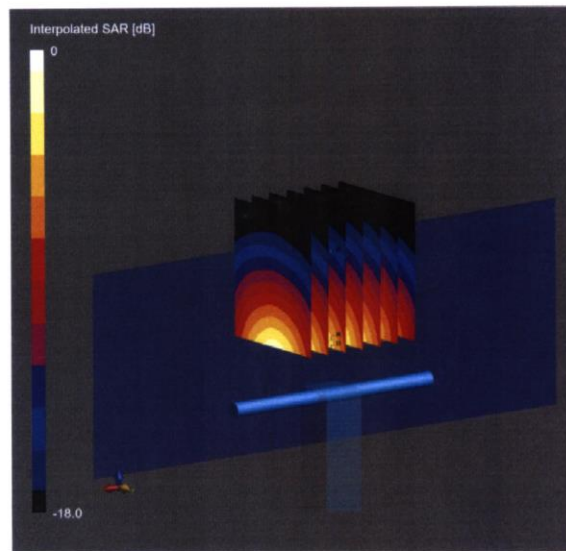
0 dB = 23.7 W/Kg
