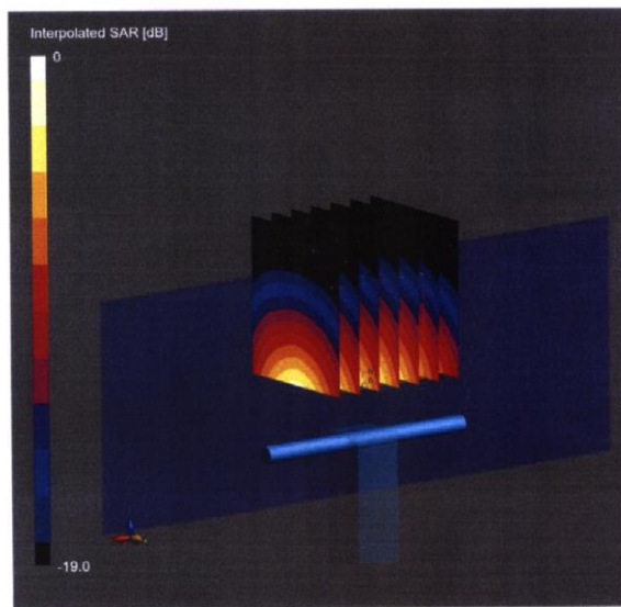
0 dB = 29.3 W/Kg
