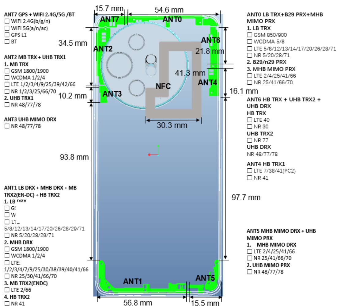
Picture 14 Antenna Locations
