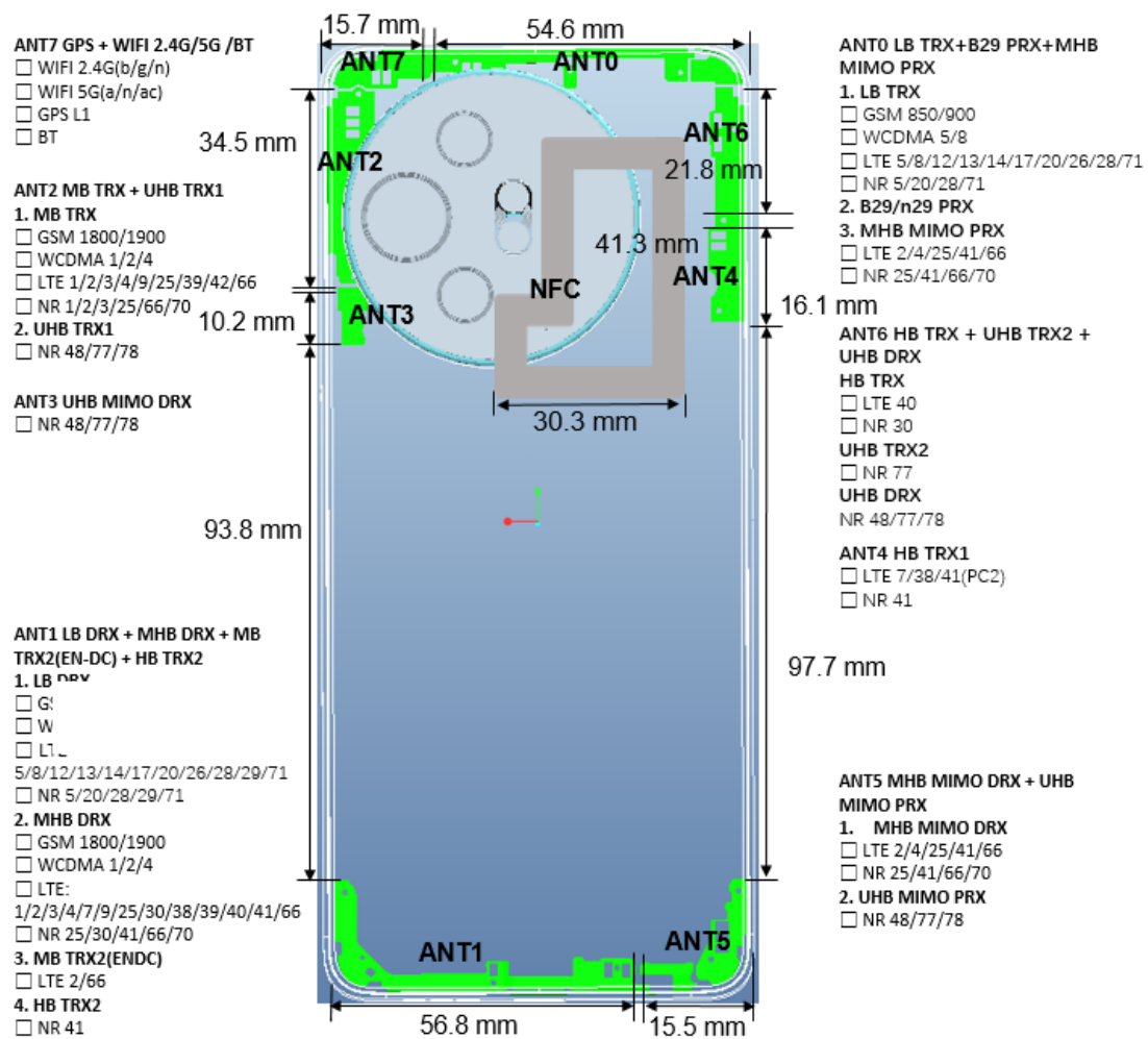
Picture 14 Antenna Locations
