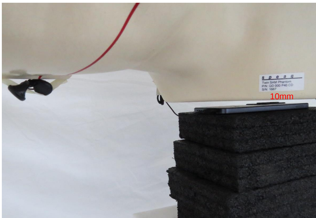
Picture 14: Back Side with Earphone, the distance from EUT to the bottom of the Phantom is 10mm
