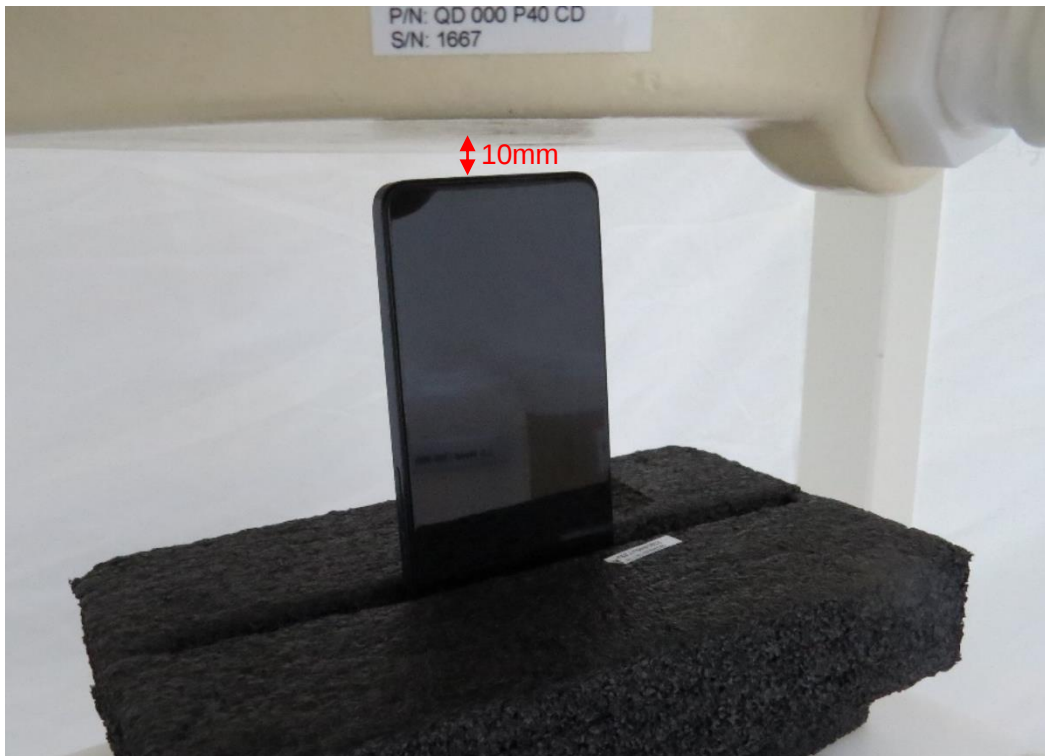
Picture 13: Bottom Edge, the distance from EUT to the bottom of the Phantom is 10mm
