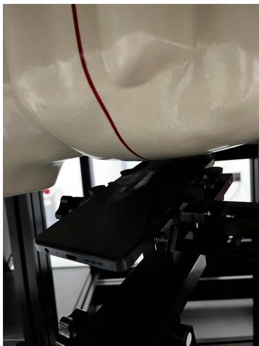
Picture 3: Left Hand Tilt 15° Position
