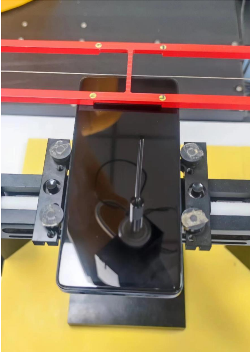
Picture 2: EUT Positioning for RF/T-coil
