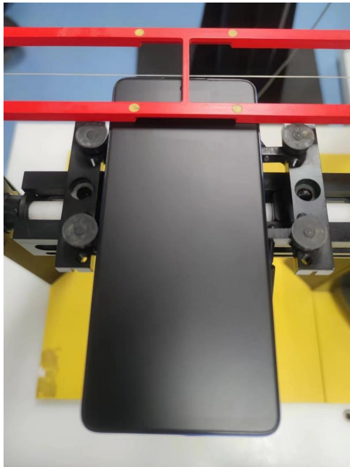
Picture 2: EUT Positioning for RF/T-coil
