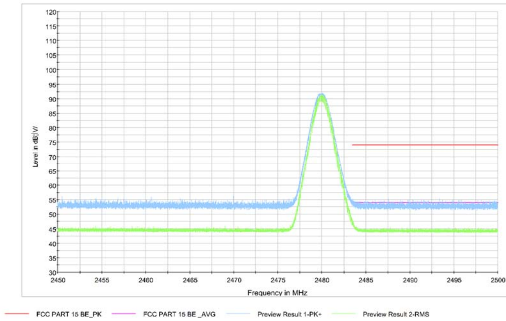
Fig.18. Frequency Band Edges: 8DPSK, Channel 78, 2.45 GHz - 2.50GHz
