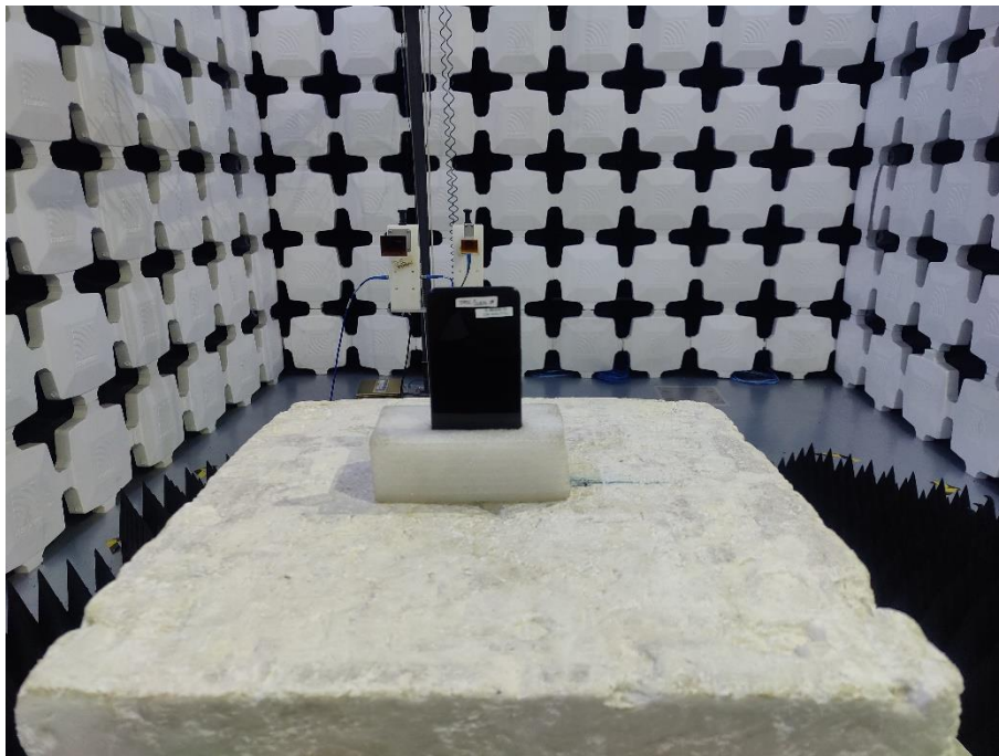
16. Radiated Emissions (Par22/24/27, 26.5GHz -40GHz)
