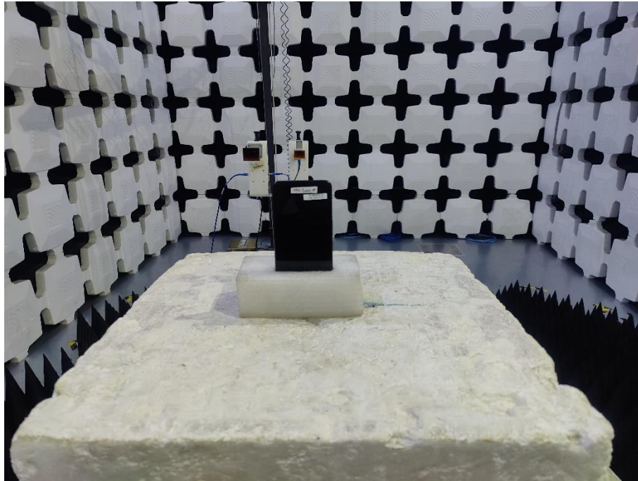
13. Radiated Emissions (Part 15C, 26.5GHz -40GHz)
