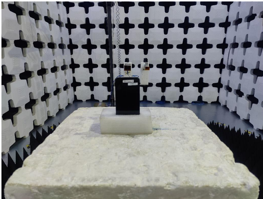
12. Radiated Emissions (Part 15C, 18GHz -26.5GHz)
