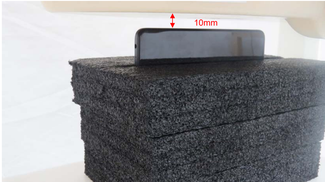
Picture 9: Left Edge, the distance from handset to the bottom of the Phantom is 10mm
