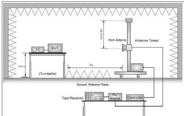
Figure 2. Above 1 GHz
