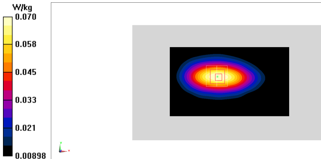
Fig.22 LTE Band5
