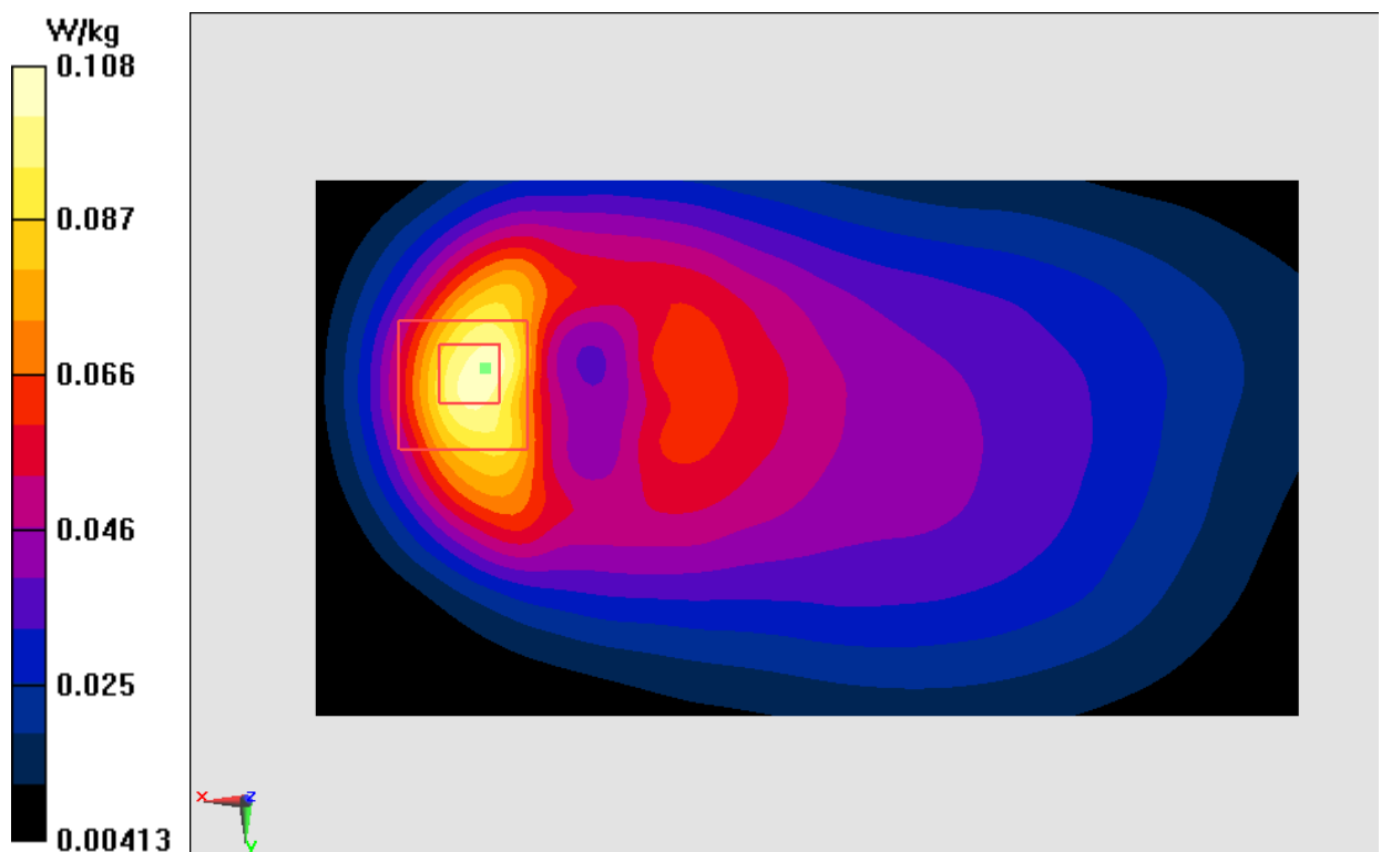
Fig.28 LTE Band12
