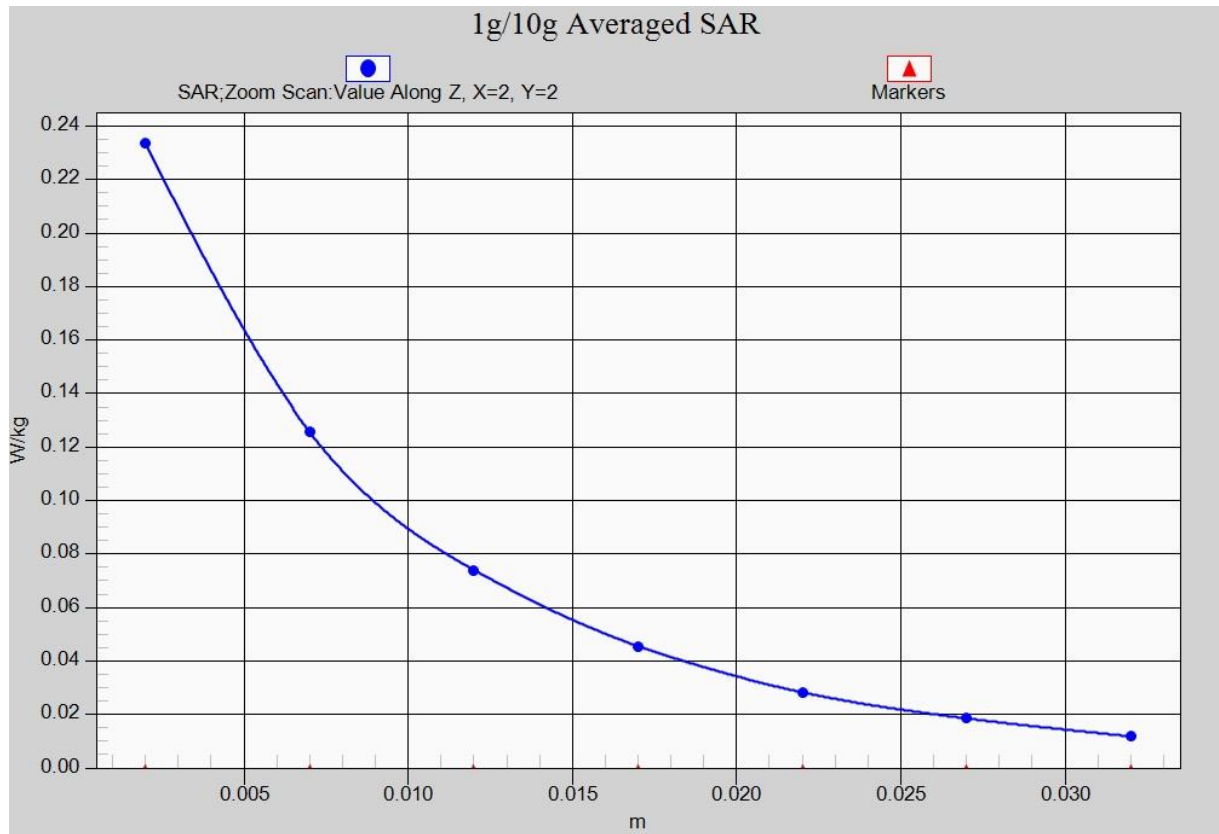
Fig. 30-1 Z-Scan at power reference point (LTE Band13)
