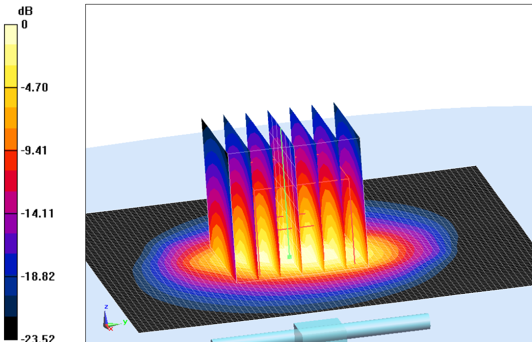
Fig.B.11 validation 2600 MHz 250mW
