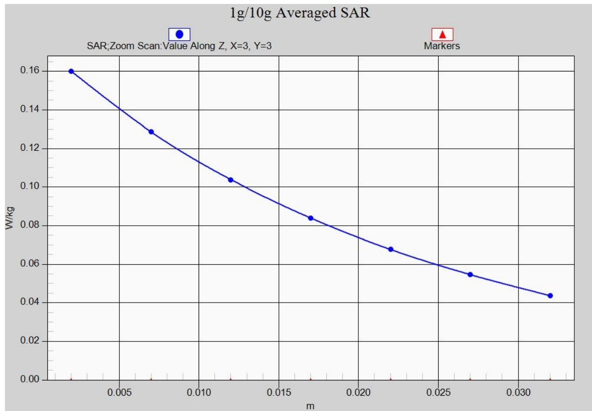
Fig. 32-1 Z-Scan at power reference point (LTE Band13)
