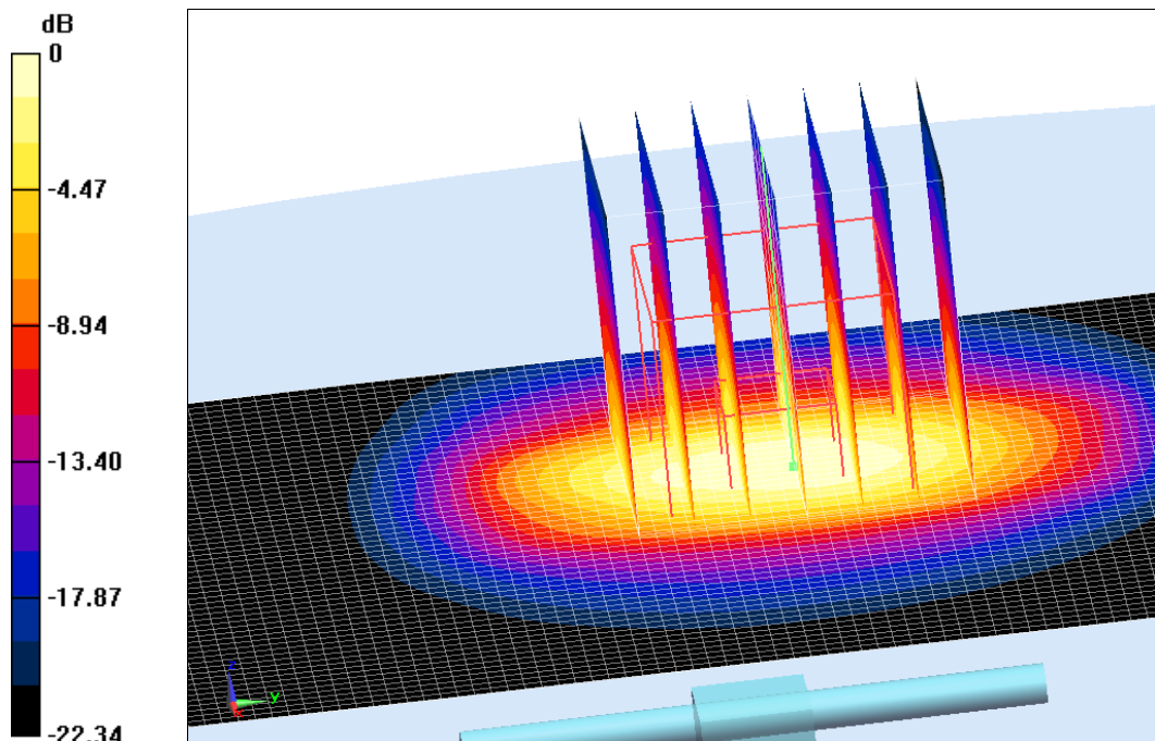
Fig.B.9 validation 2450 MHz 250mW
