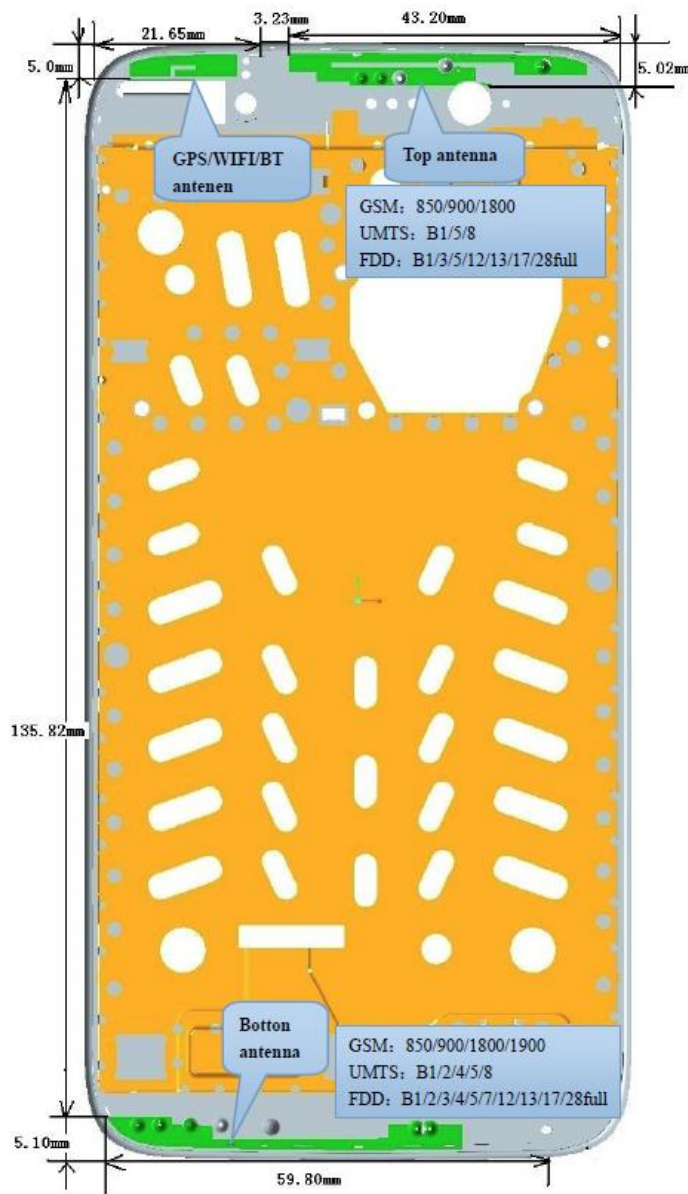
Picture 12.1 Antenna Locations
