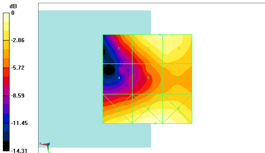
Fig B.6 HAC RF E-Field GSM 1900 Low
