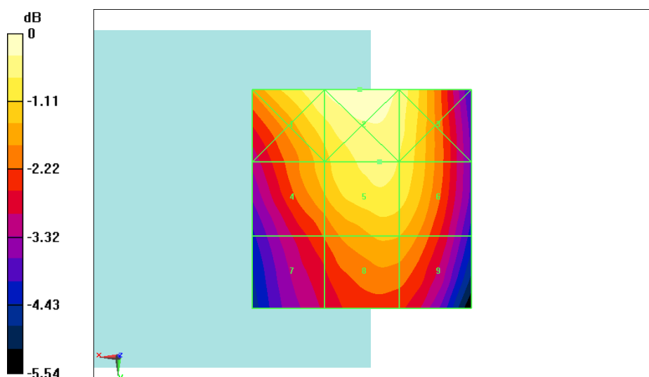
Fig B.2 HAC RF E-Field GSM 850 Middle
