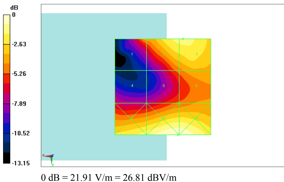
Fig B.4 HAC RF E-Field GSM 1900 High
