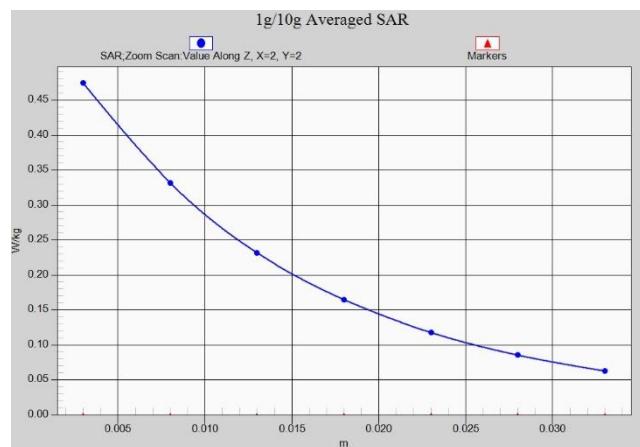
Fig.A.1- 23 Z-Scan at power reference point (LTE band66)
