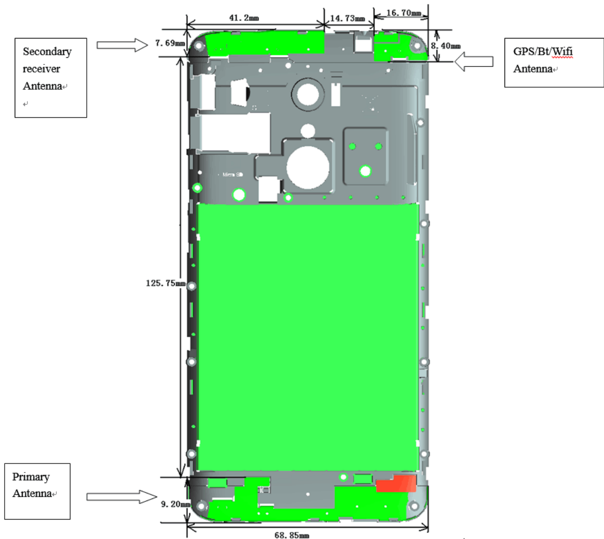
Picture 12.1 Antenna Locations
