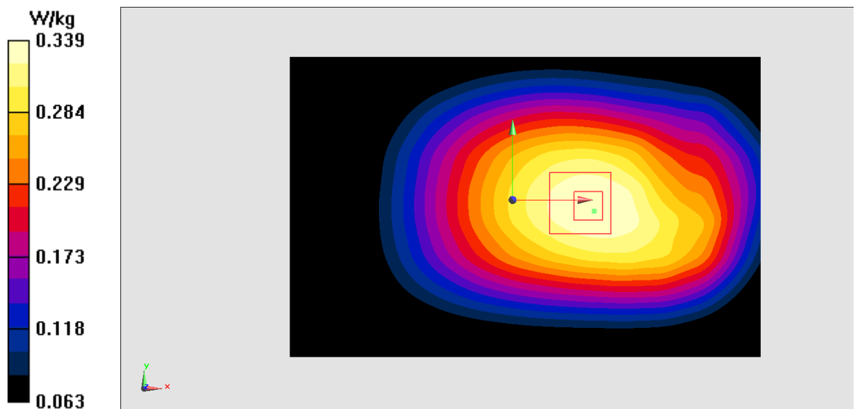
Fig.18 LTE Band12
