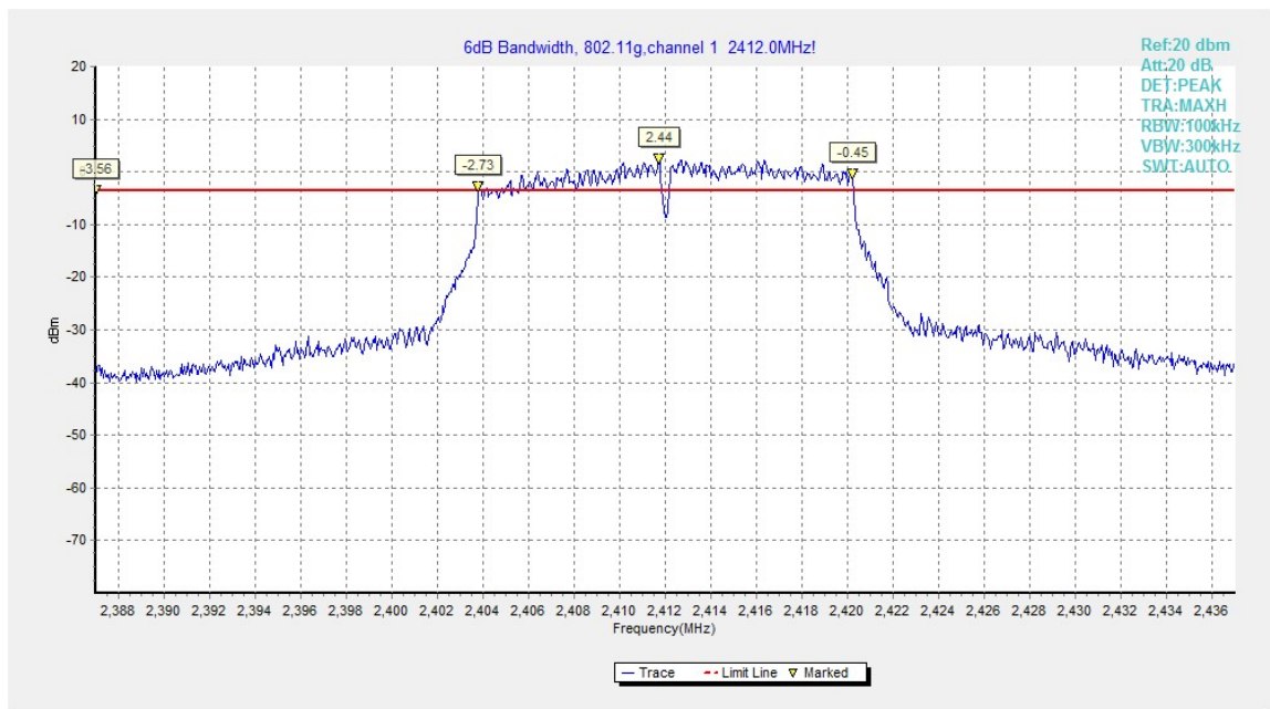
Fig.A.4.4 Occupied 6dB Bandwidth (802.11g, Ch 1)
