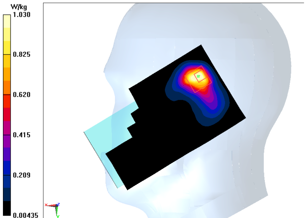
Fig.21 2450 MHz
