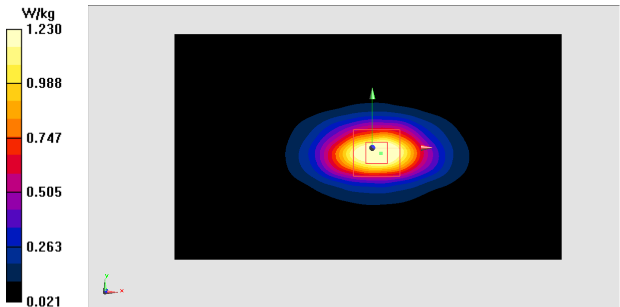
Fig.8 1700 MHz
