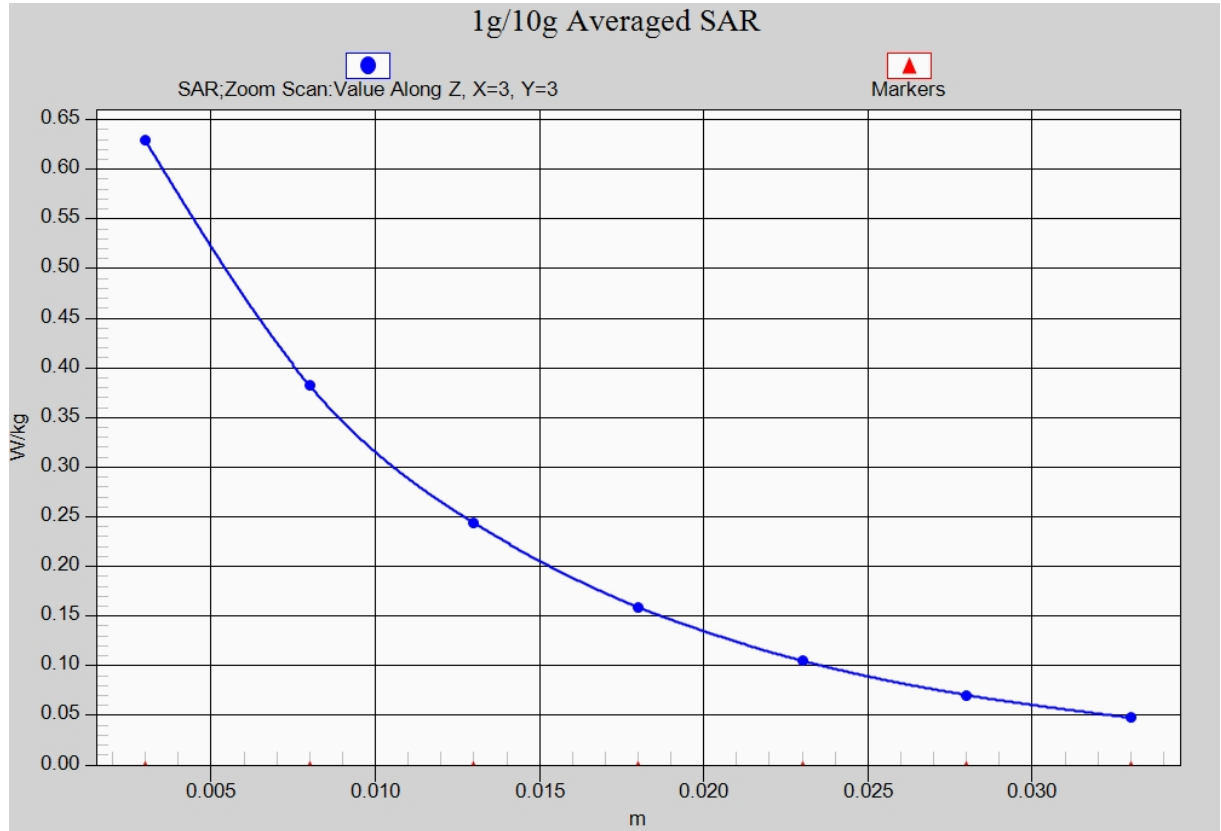
Fig. 20-1 Z-Scan at power reference point (LTE Band17)
