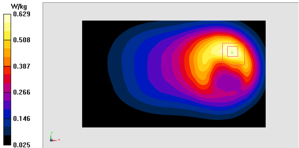
Fig.20 LTE Band17
