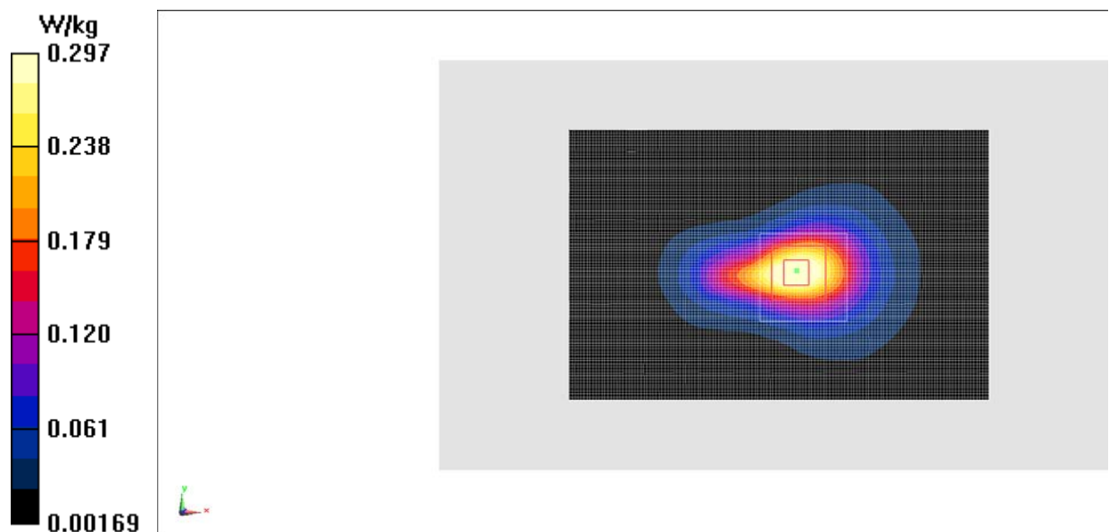
Fig.22 2450 MHz
