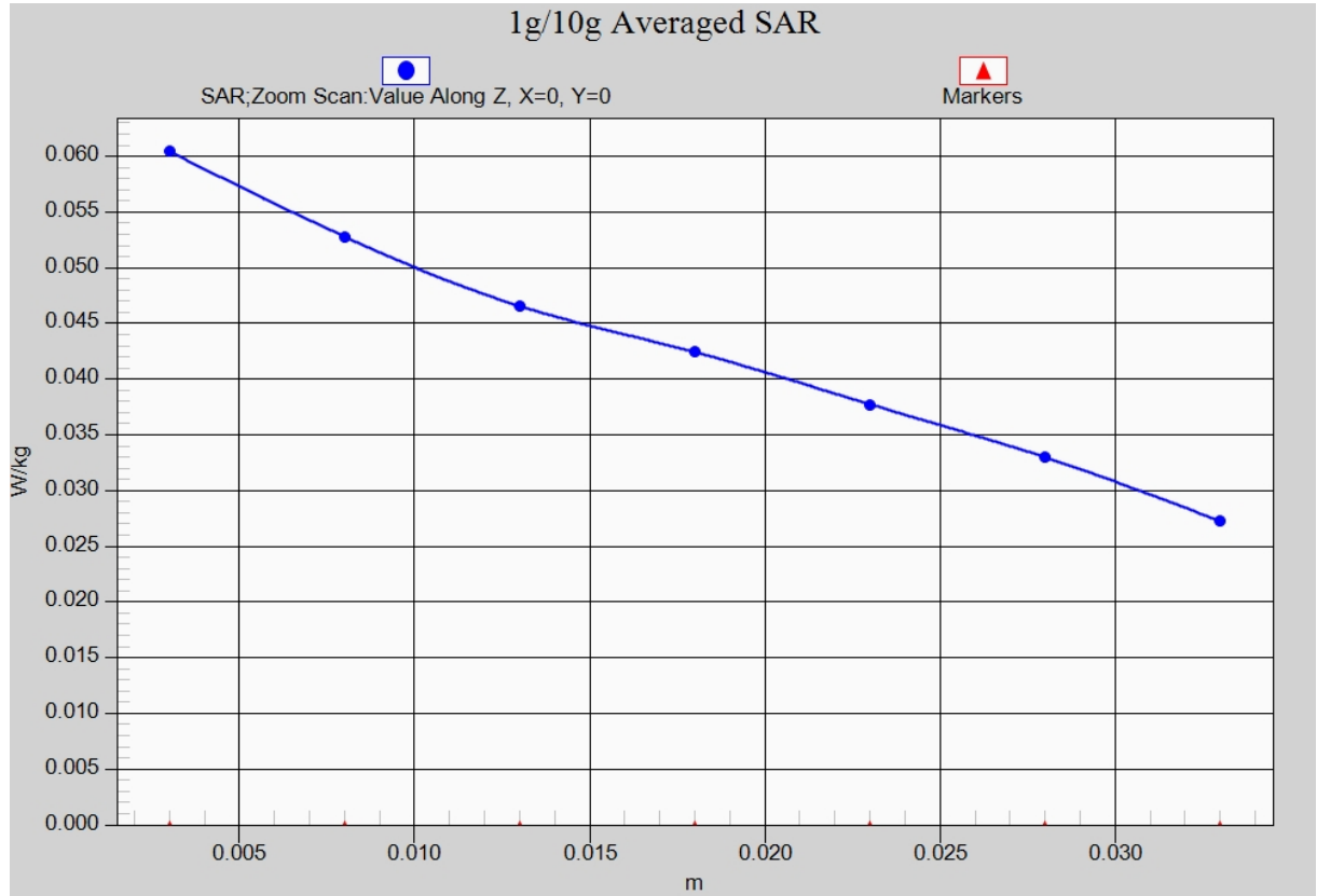
Fig. 19-1 Z-Scan at power reference point (LTE Band17)
