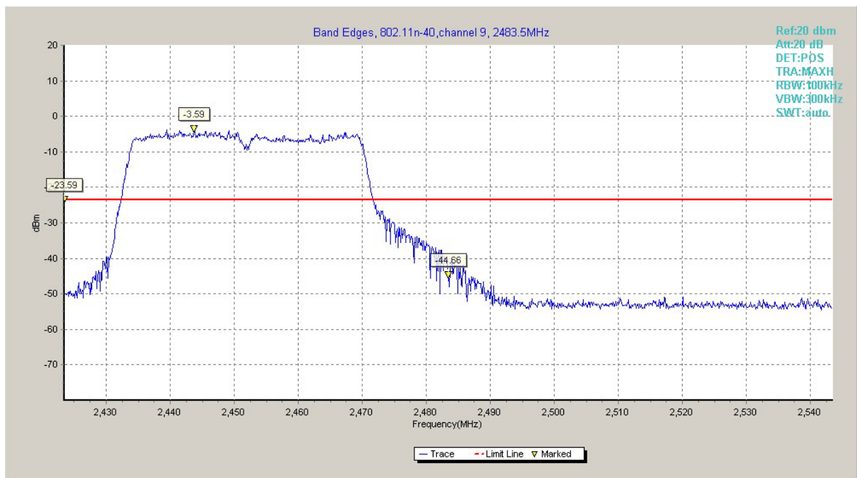
Fig.A.5.14 Band Edges (802.11n-HT40, Ch 9)
