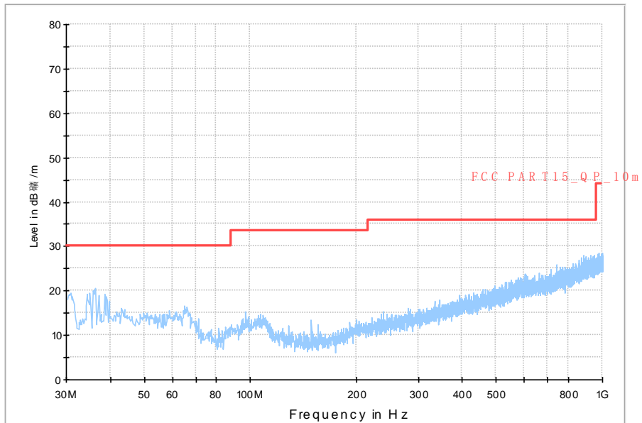
Normal RE_30M-1GHz_10m
