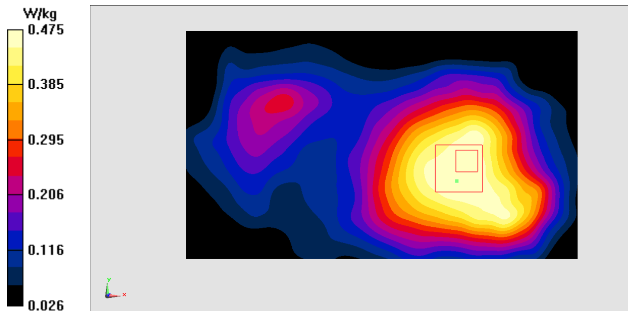
Fig.18 1700 MHz
