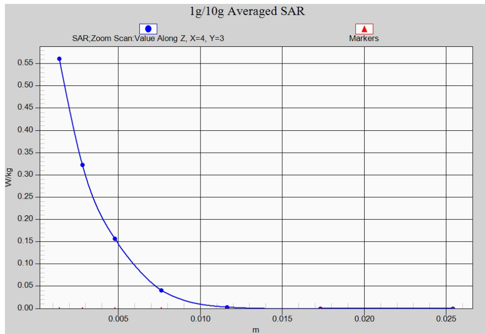
Fig. 28-1 Z-Scan at power reference point (5GHz)
