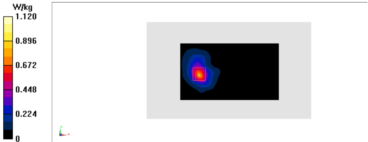
Fig.28 5GHz
