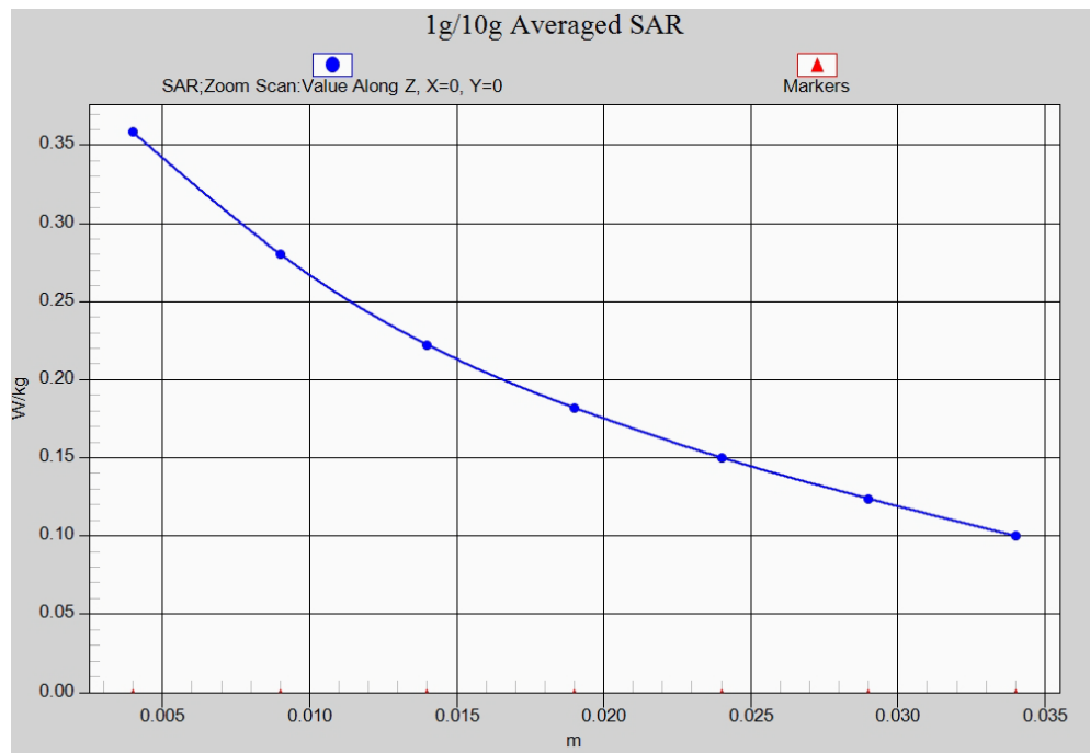
Fig. 20-1 Z-Scan at power reference point (LTE Band5)
