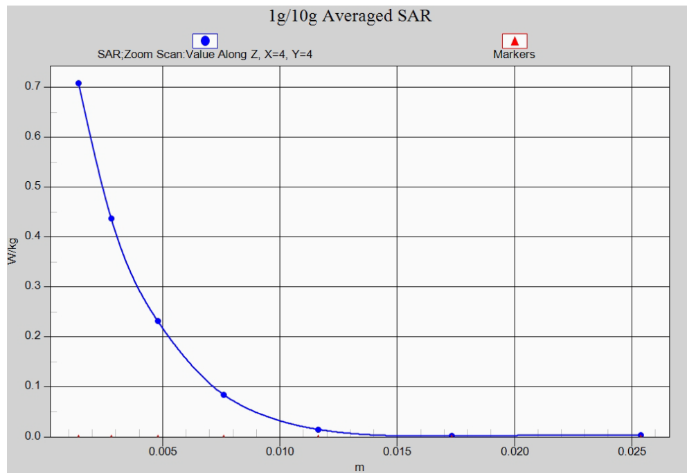
Fig. 26-1 Z-Scan at power reference point (5GHz)
