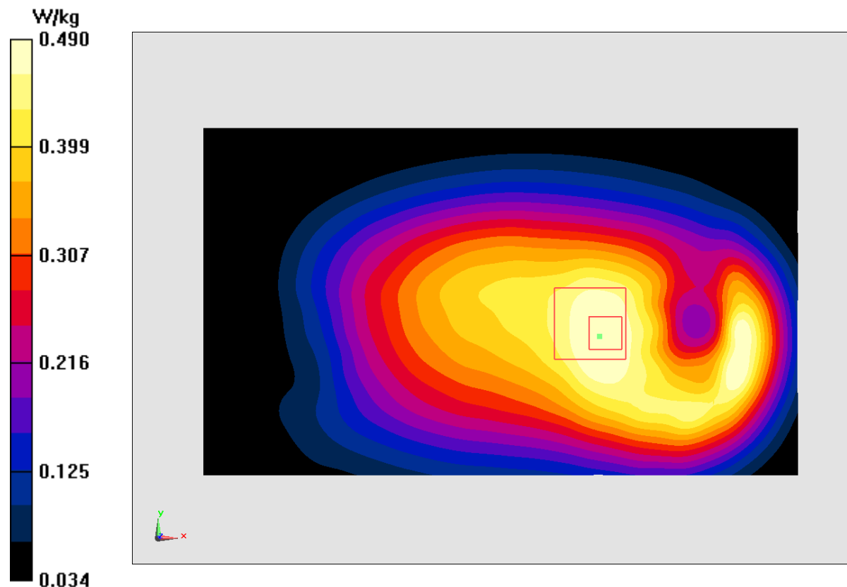
Fig.22 LTE Band5
