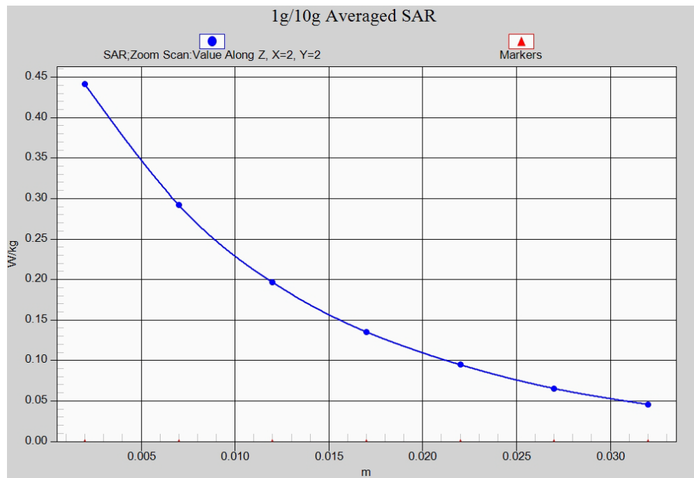
Fig. 17-1 Z-Scan at power reference point (1700 MHz)
