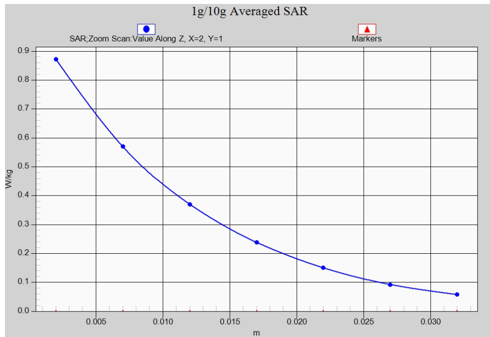
Fig.18-1 Z-Scan at power reference point (1700 MHz)
