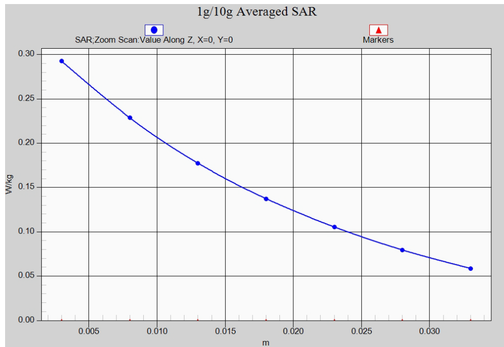
Fig. 19-1 Z-Scan at power reference point (LTE Band5)
