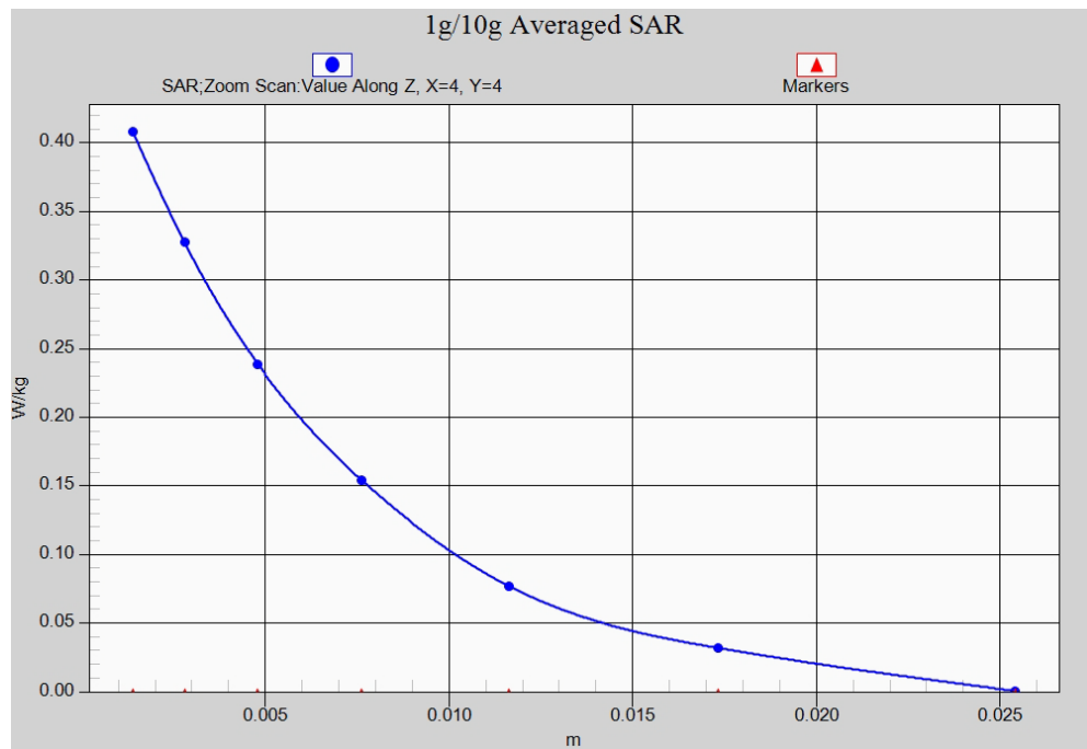
Fig. 27-1 Z-Scan at power reference point (5GHz)
