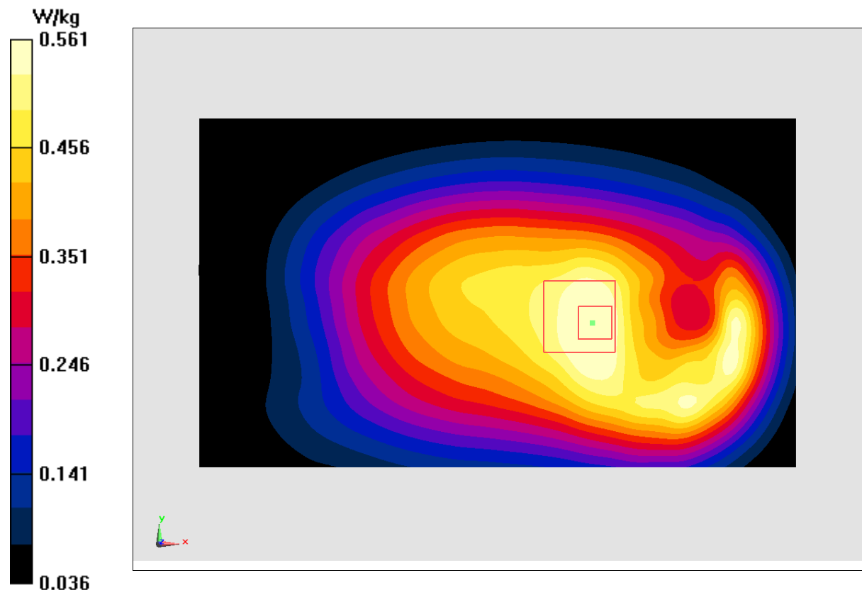
Fig.20 LTE Band5
