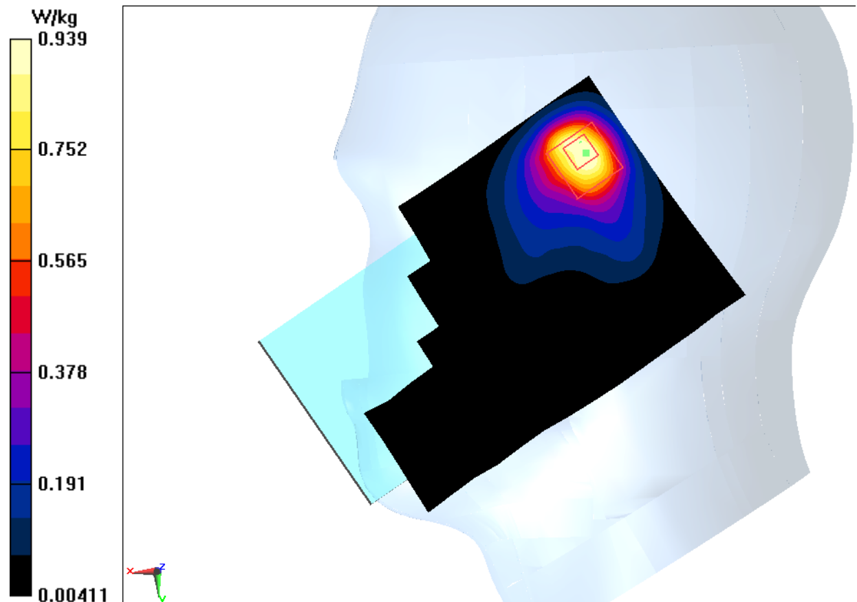
Fig.23 2450 MHz
