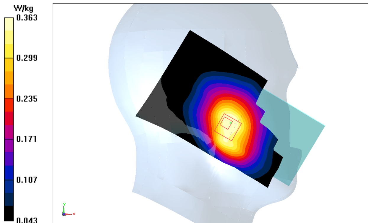
Fig.1 850MHz
