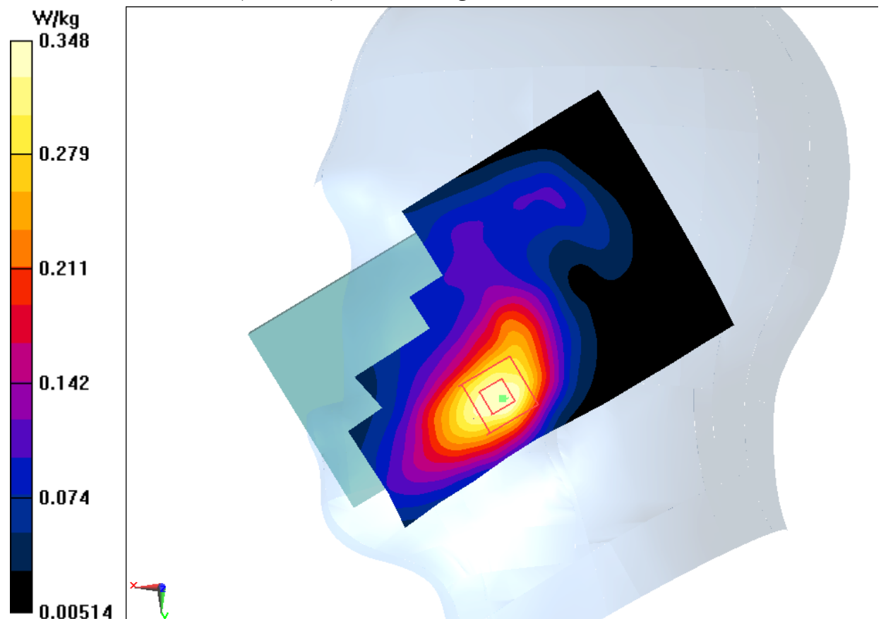
Fig.9 LTE Band2
