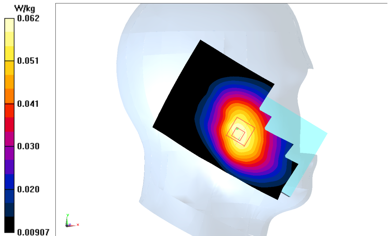
Fig.15 LTE Band17
