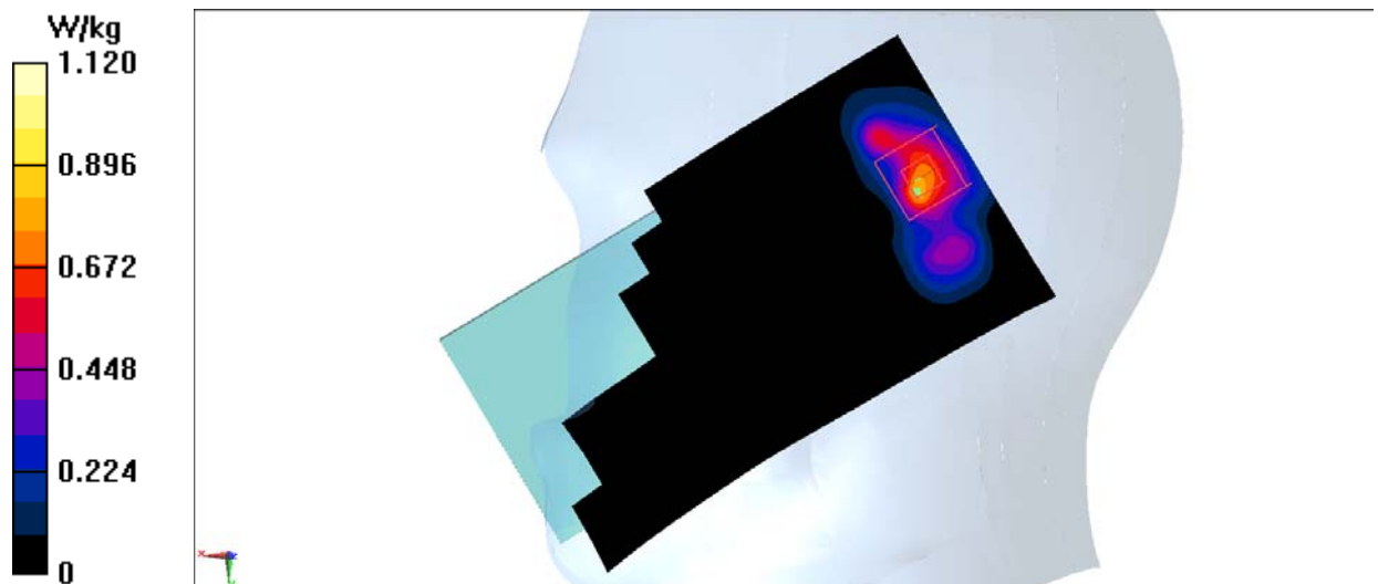
Fig.23 5GHz
