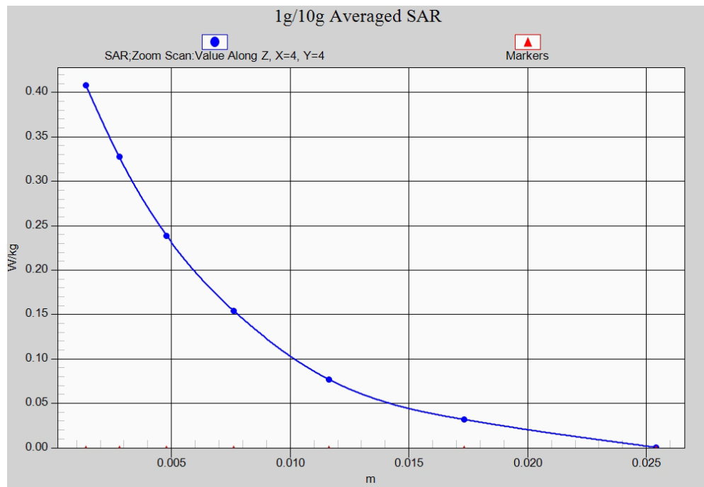
Fig. 23-1 Z-Scan at power reference point (5GHz)
