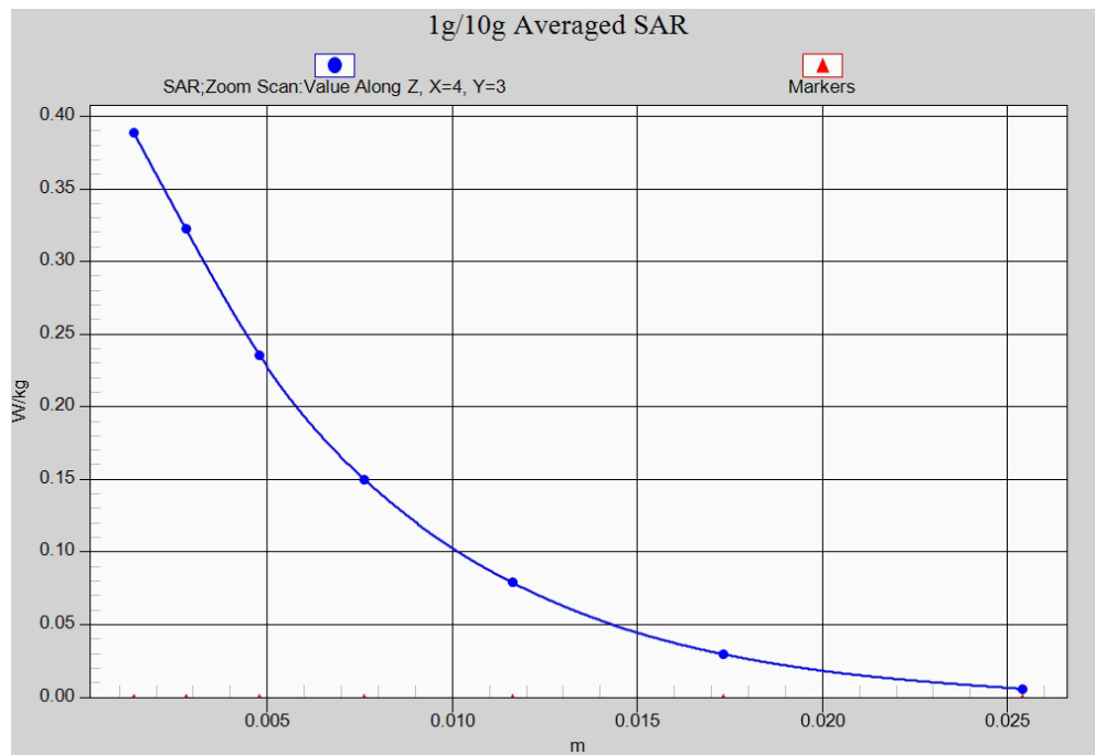
Fig. 21-1 Z-Scan at power reference point (5GHz)
