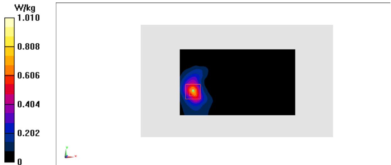
Fig.22 5GHz
