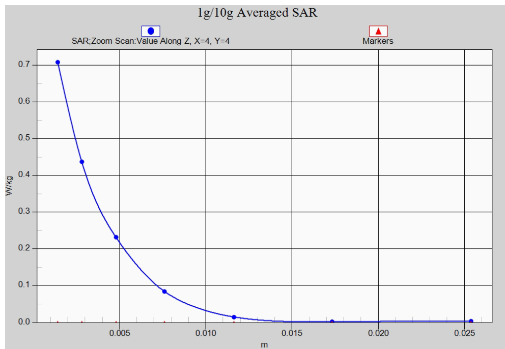
Fig. 22-1 Z-Scan at power reference point (5GHz)
