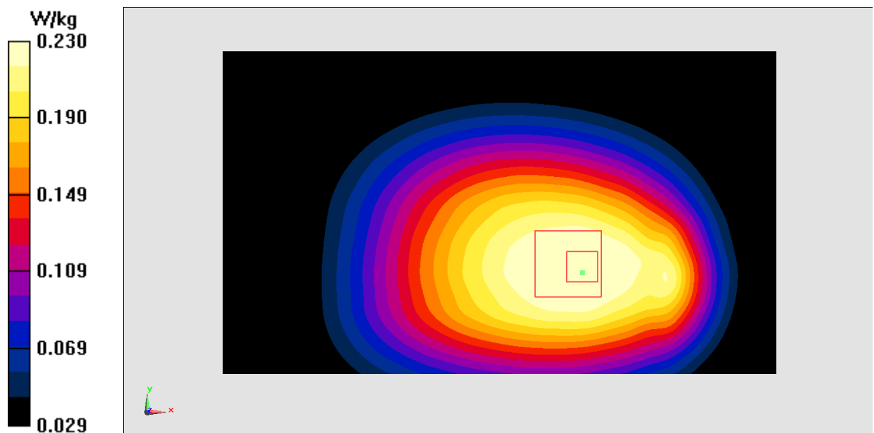
Fig.18 LTE Band17
