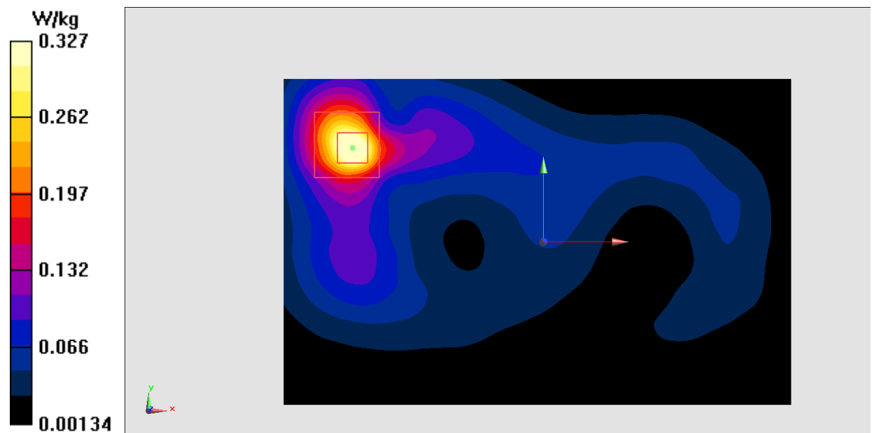
Fig.20 2450 MHz
