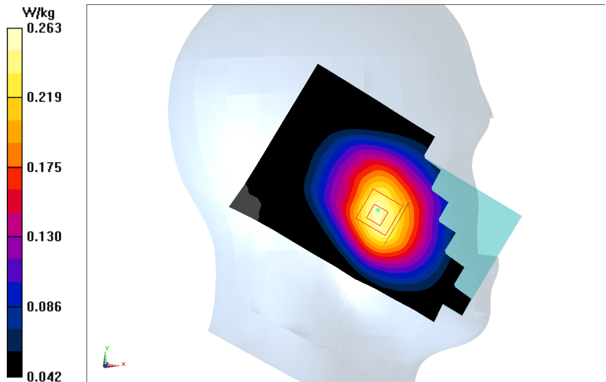
Fig.15 LTE Band 13
